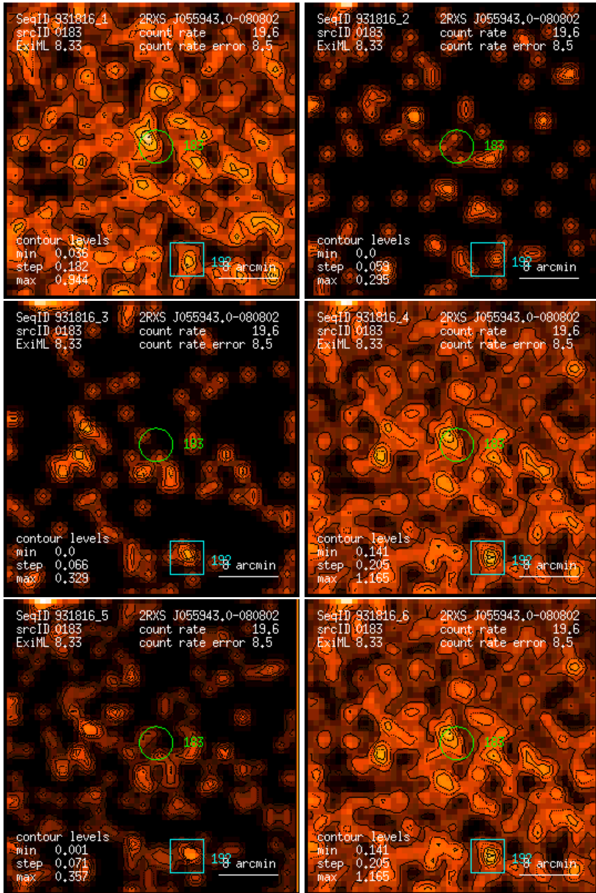
Figure 183: RASS 931816: detection 0183: band rate images, Gaussian filter: (1) PSPC channels 11 – 41, (2) 52 – 90, (3) 91 – 201, (4) 11 – 235, (5) 52 – 201, (6) 11 – 201. Broad band rates in counts/ks. Band rate contour levels in counts/ks/arcmin 2 .
