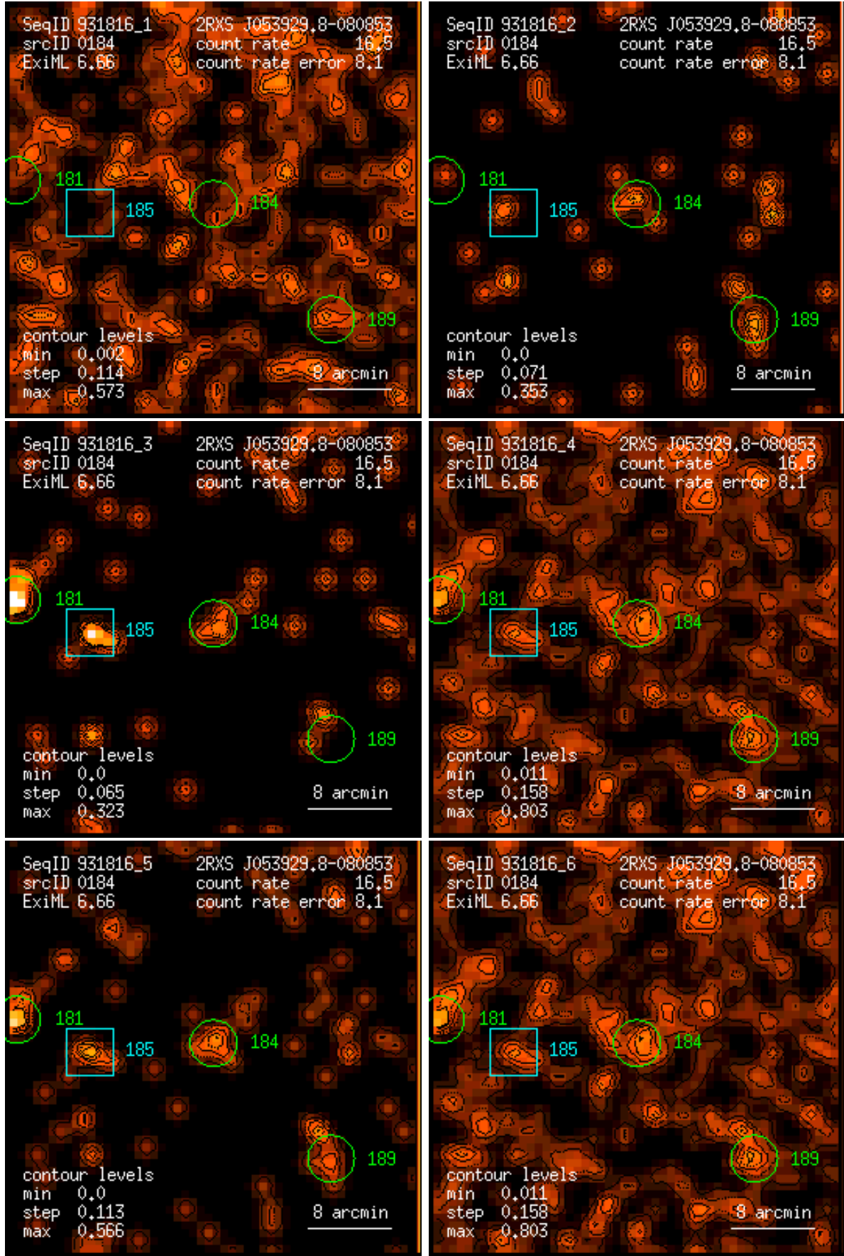
Figure 184: RASS 931816: detection 0184: band rate images, Gaussian filter: (1) PSPC channels 11 – 41, (2) 52 – 90, (3) 91 – 201, (4) 11 – 235, (5) 52 – 201, (6) 11 – 201. Broad band rates in counts/ks. Band rate contour levels in counts/ks/arcmin 2 .
