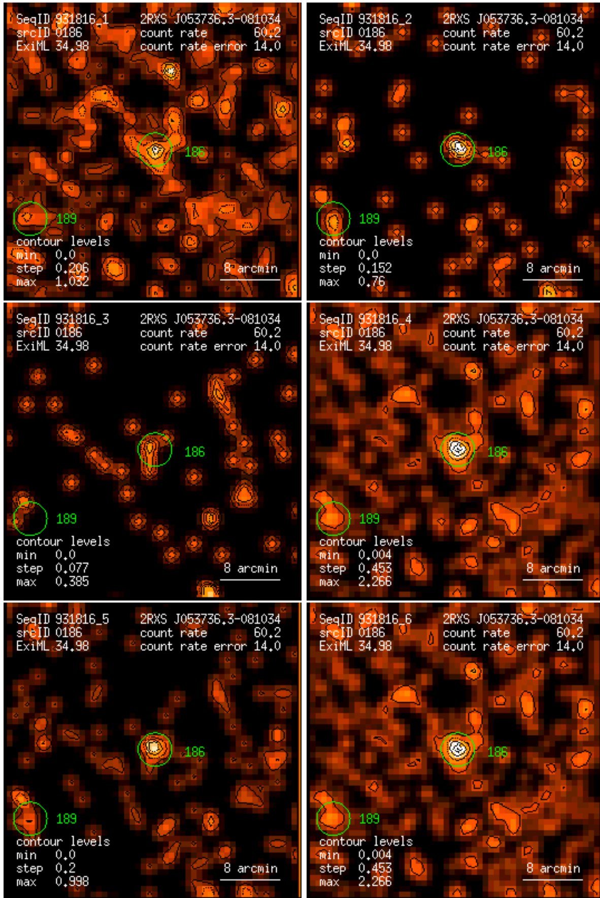
Figure 186: RASS 931816: detection 0186: band rate images, Gaussian filter: (1) PSPC channels 11 – 41, (2) 52 – 90, (3) 91 – 201, (4) 11 – 235, (5) 52 – 201, (6) 11 – 201. Broad band rates in counts/ks. Band rate contour levels in counts/ks/arcmin 2 .
