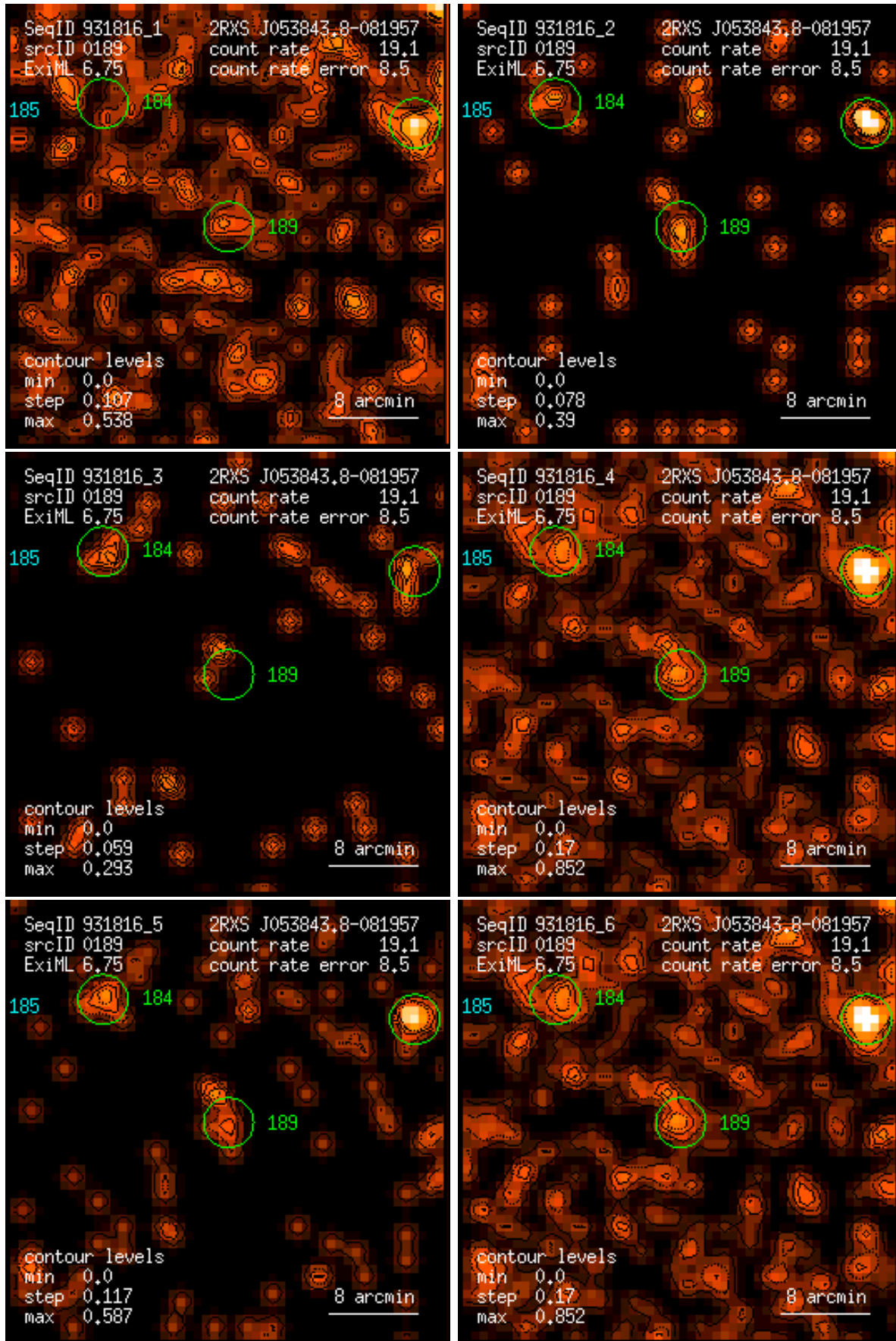
Figure 189: RASS 931816: detection 0189: band rate images, Gaussian filter: (1) PSPC channels 11 – 41, (2) 52 – 90, (3) 91 – 201, (4) 11 – 235, (5) 52 – 201, (6) 11 – 201. Broad band rates in counts/ks. Band rate contour levels in counts/ks/arcmin 2 .
