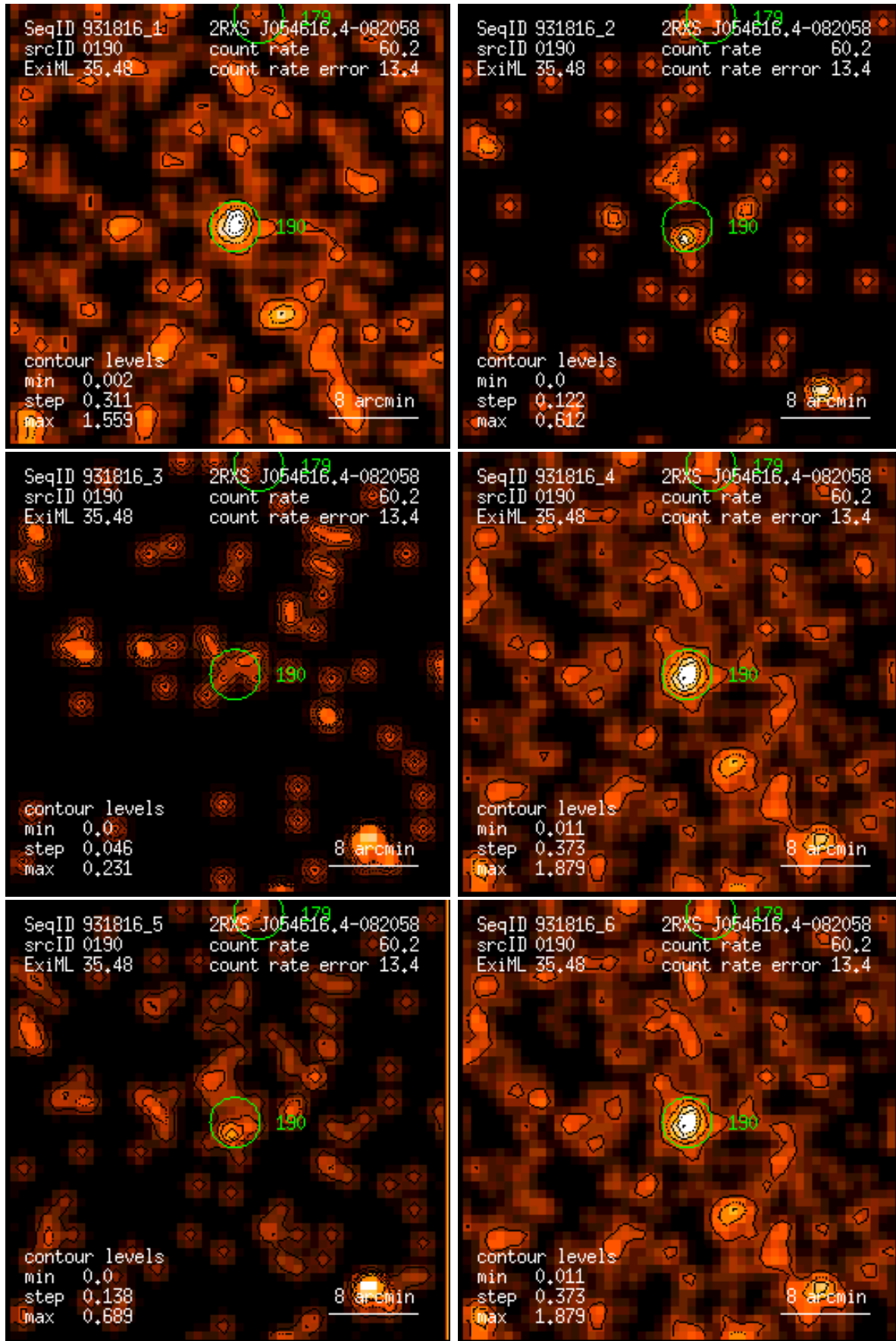
Figure 190: RASS 931816: detection 0190: band rate images, Gaussian filter: (1) PSPC channels 11 – 41, (2) 52 – 90, (3) 91 – 201, (4) 11 – 235, (5) 52 – 201, (6) 11 – 201. Broad band rates in counts/ks. Band rate contour levels in counts/ks/arcmin 2 .
