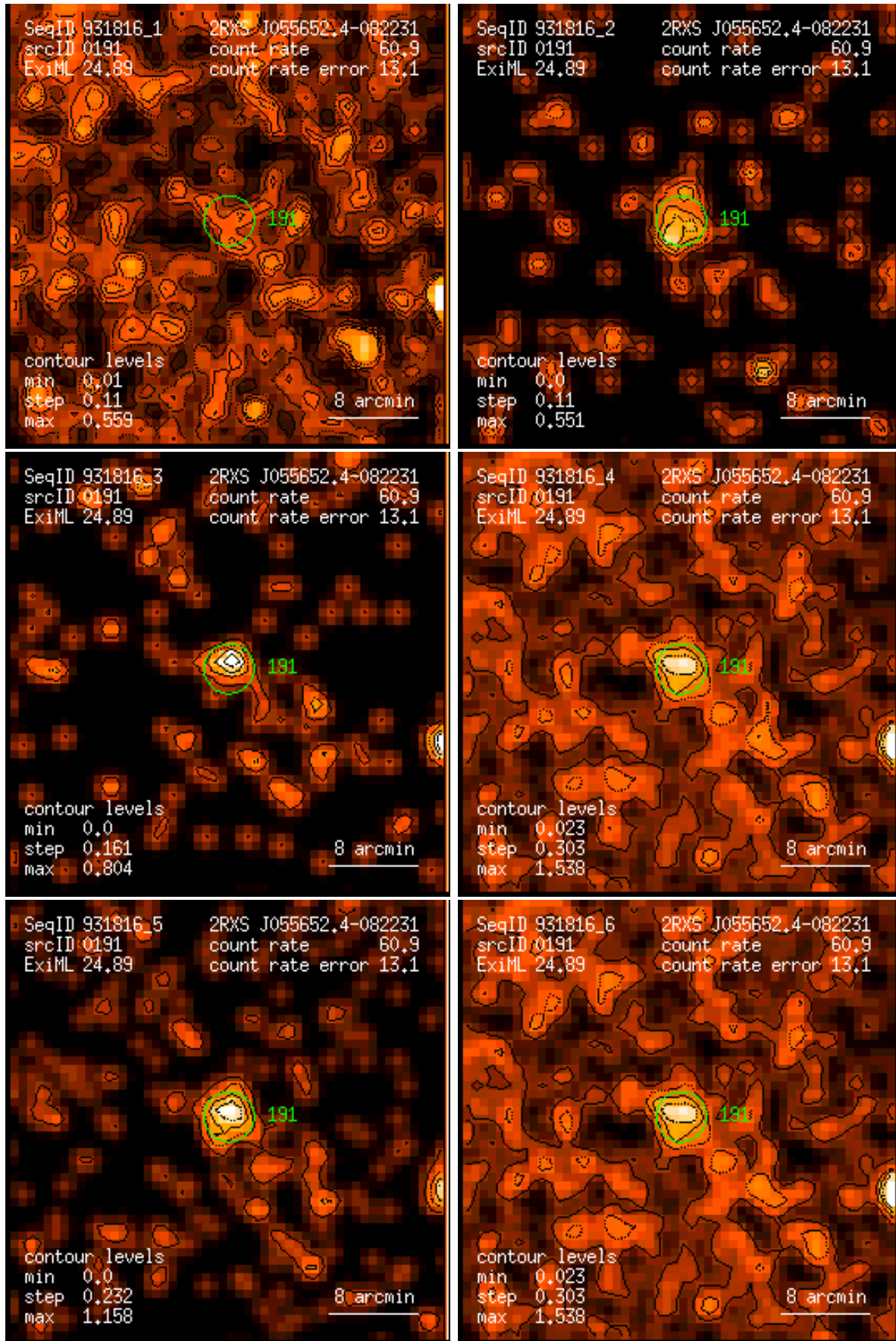
Figure 191: RASS 931816: detection 0191: band rate images, Gaussian filter: (1) PSPC channels 11 – 41, (2) 52 – 90, (3) 91 – 201, (4) 11 – 235, (5) 52 – 201, (6) 11 – 201. Broad band rates in counts/ks. Band rate contour levels in counts/ks/arcmin 2 .
