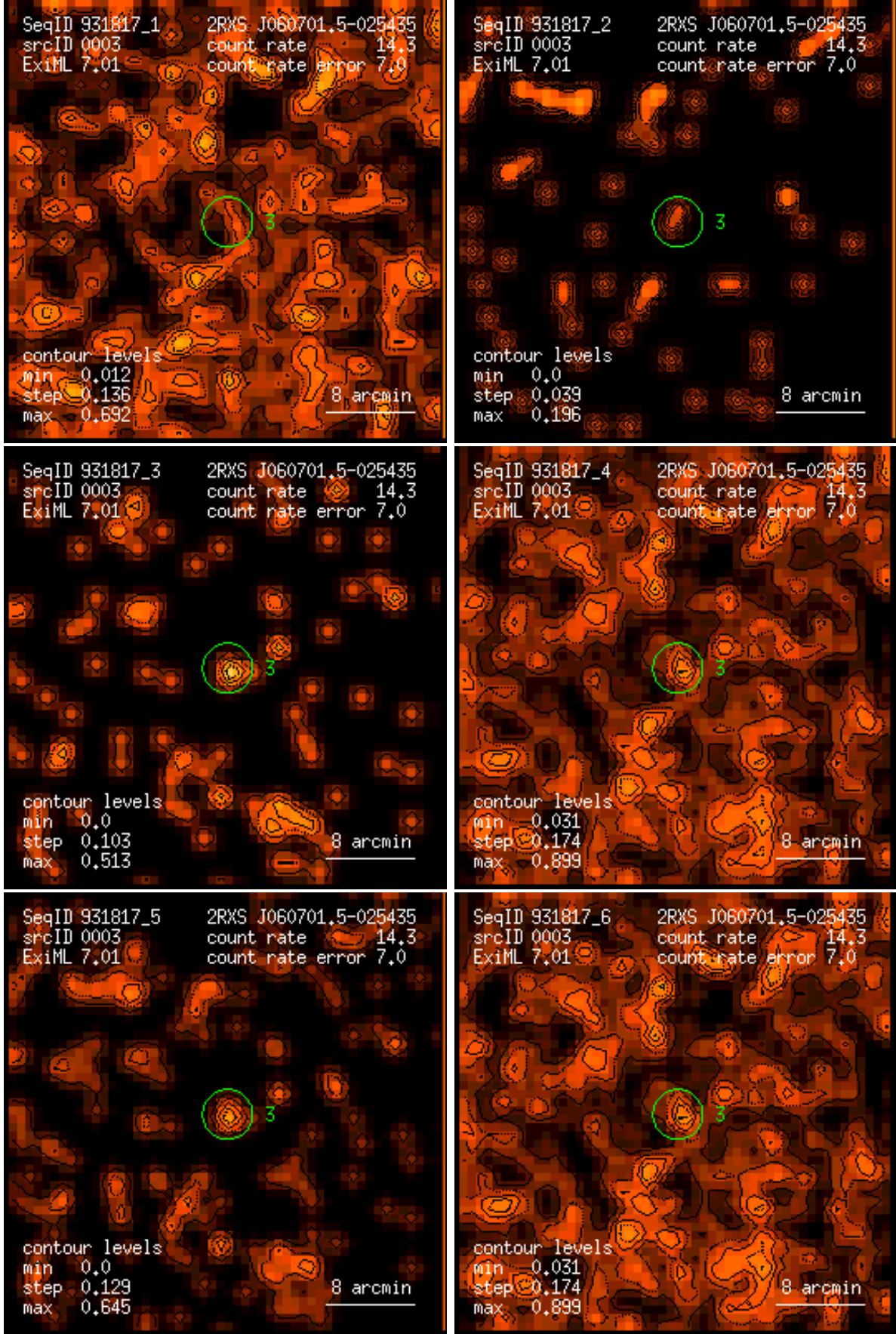
Figure 3: RASS 931817: detection 0003: band rate images, Gaussian filter: (1) PSPC channels 11 – 41, (2) 52 – 90, (3) 91 – 201, (4) 11 – 235, (5) 52 – 201, (6) 11 – 201. Broad band rates in counts/ks. Band rate contour levels in counts/ks/arcmin 2 .
