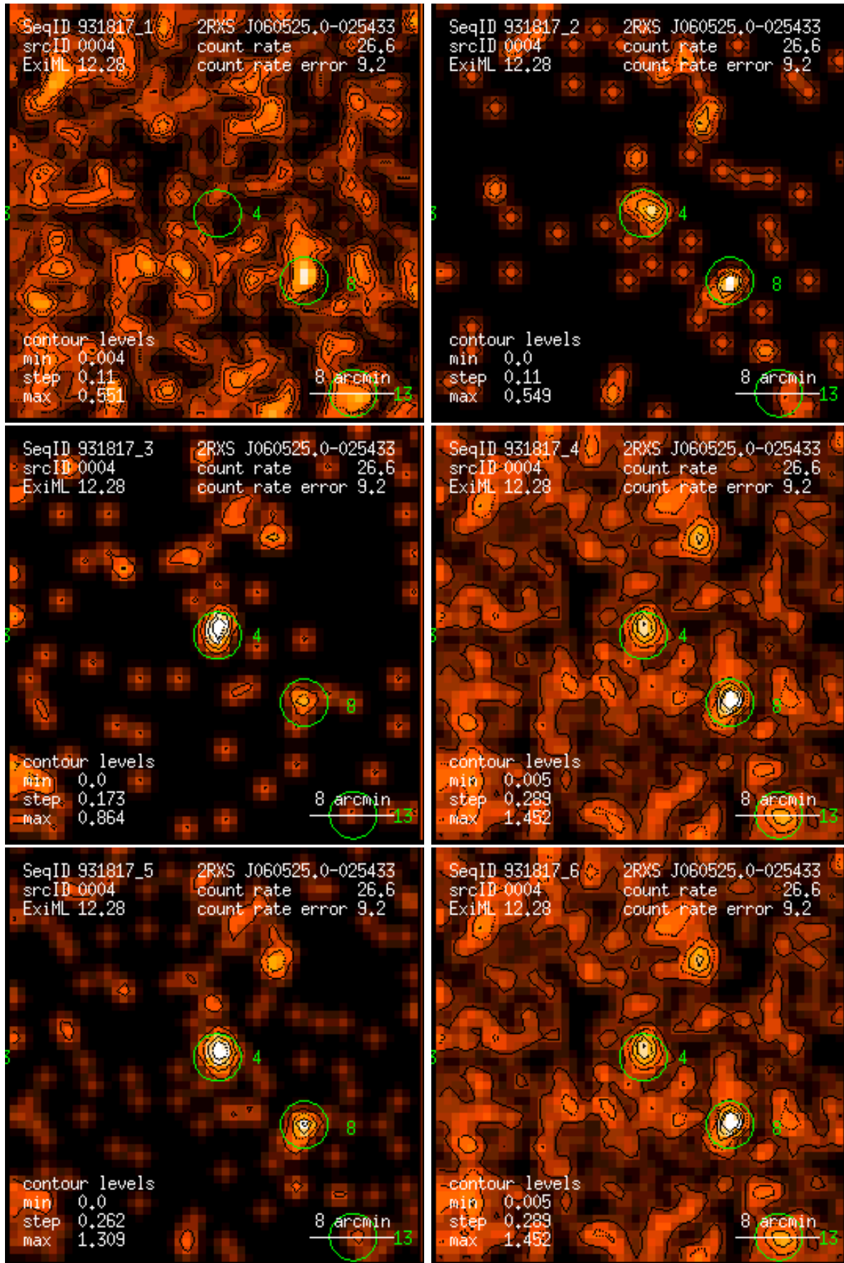
Figure 4: RASS 931817: detection 0004: band rate images, Gaussian filter: (1) PSPC channels 11 – 41, (2) 52 – 90, (3) 91 – 201, (4) 11 – 235, (5) 52 – 201, (6) 11 – 201. Broad band rates in counts/ks. Band rate contour levels in counts/ks/arcmin 2 .
