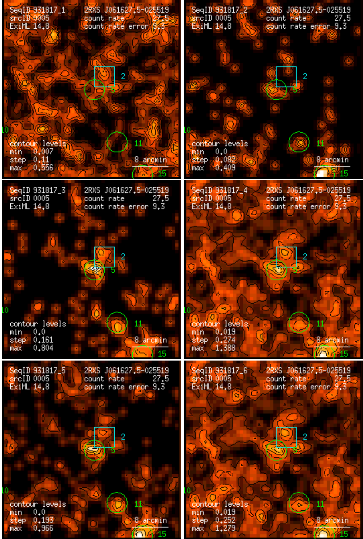
Figure 5: RASS 931817: detection 0005: band rate images, Gaussian filter: (1) PSPC channels 11 – 41, (2) 52 – 90, (3) 91 – 201, (4) 11 – 235, (5) 52 – 201, (6) 11 – 201. Broad band rates in counts/ks. Band rate contour levels in counts/ks/arcmin 2 .
