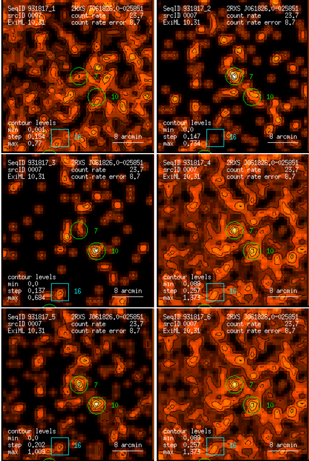
Figure 7: RASS 931817: detection 0007: band rate images, Gaussian filter: (1) PSPC channels 11 – 41, (2) 52 – 90, (3) 91 – 201, (4) 11 – 235, (5) 52 – 201, (6) 11 – 201. Broad band rates in counts/ks. Band rate contour levels in counts/ks/arcmin 2 .
