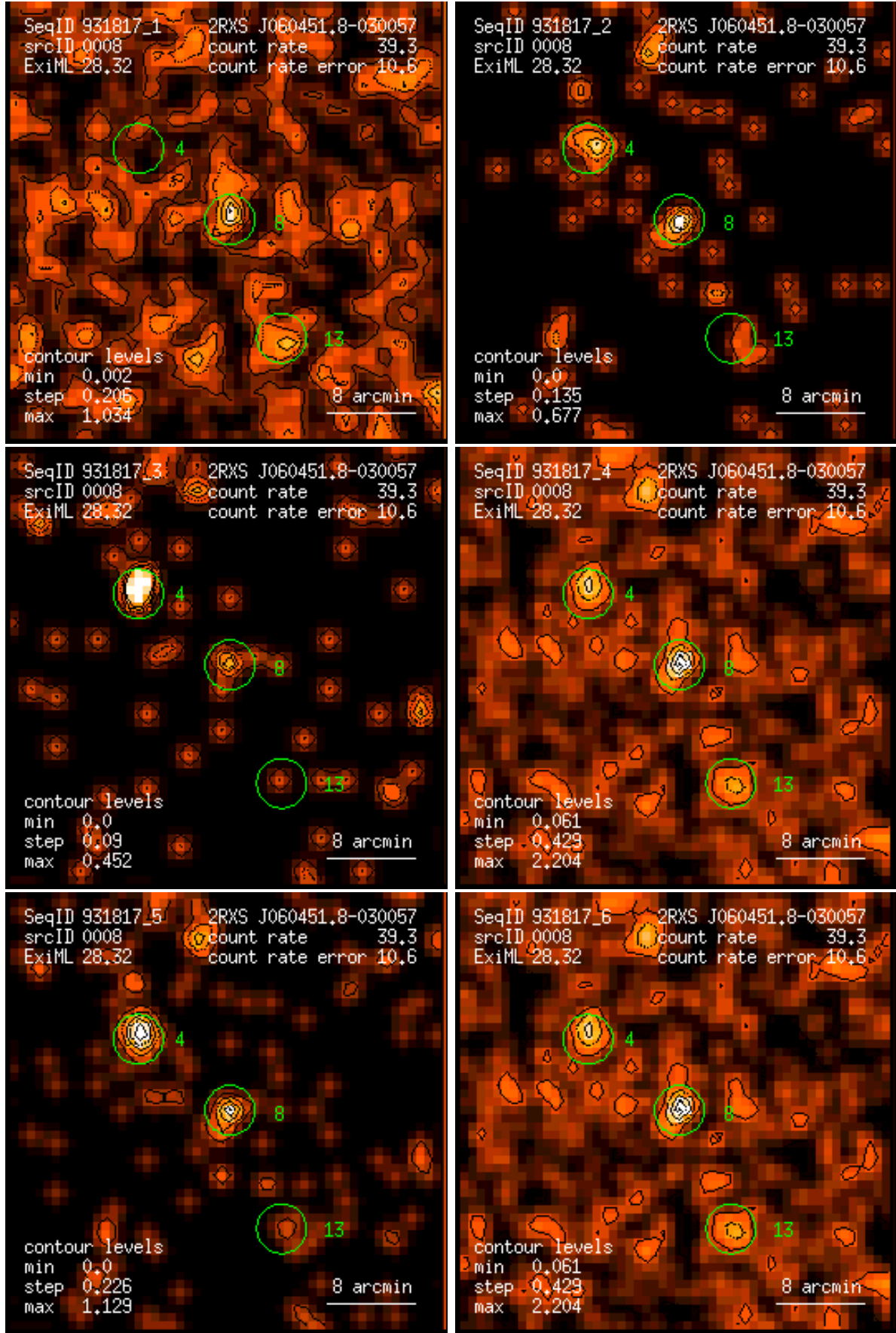
Figure 8: RASS 931817: detection 0008: band rate images, Gaussian filter: (1) PSPC channels 11 – 41, (2) 52 – 90, (3) 91 – 201, (4) 11 – 235, (5) 52 – 201, (6) 11 – 201. Broad band rates in counts/ks. Band rate contour levels in counts/ks/arcmin 2 .
