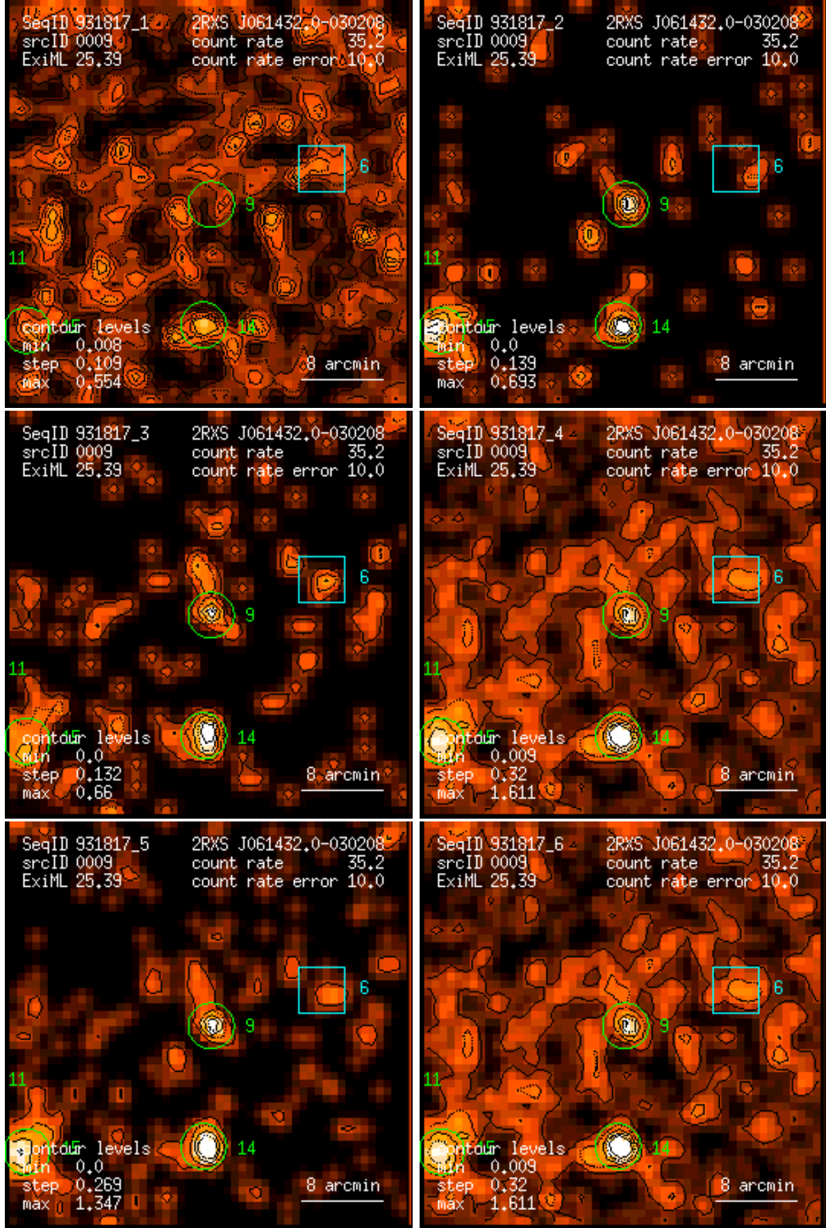
Figure 9: RASS 931817: detection 0009: band rate images, Gaussian filter: (1) PSPC channels 11 – 41, (2) 52 – 90, (3) 91 – 201, (4) 11 – 235, (5) 52 – 201, (6) 11 – 201. Broad band rates in counts/ks. Band rate contour levels in counts/ks/arcmin 2 .
