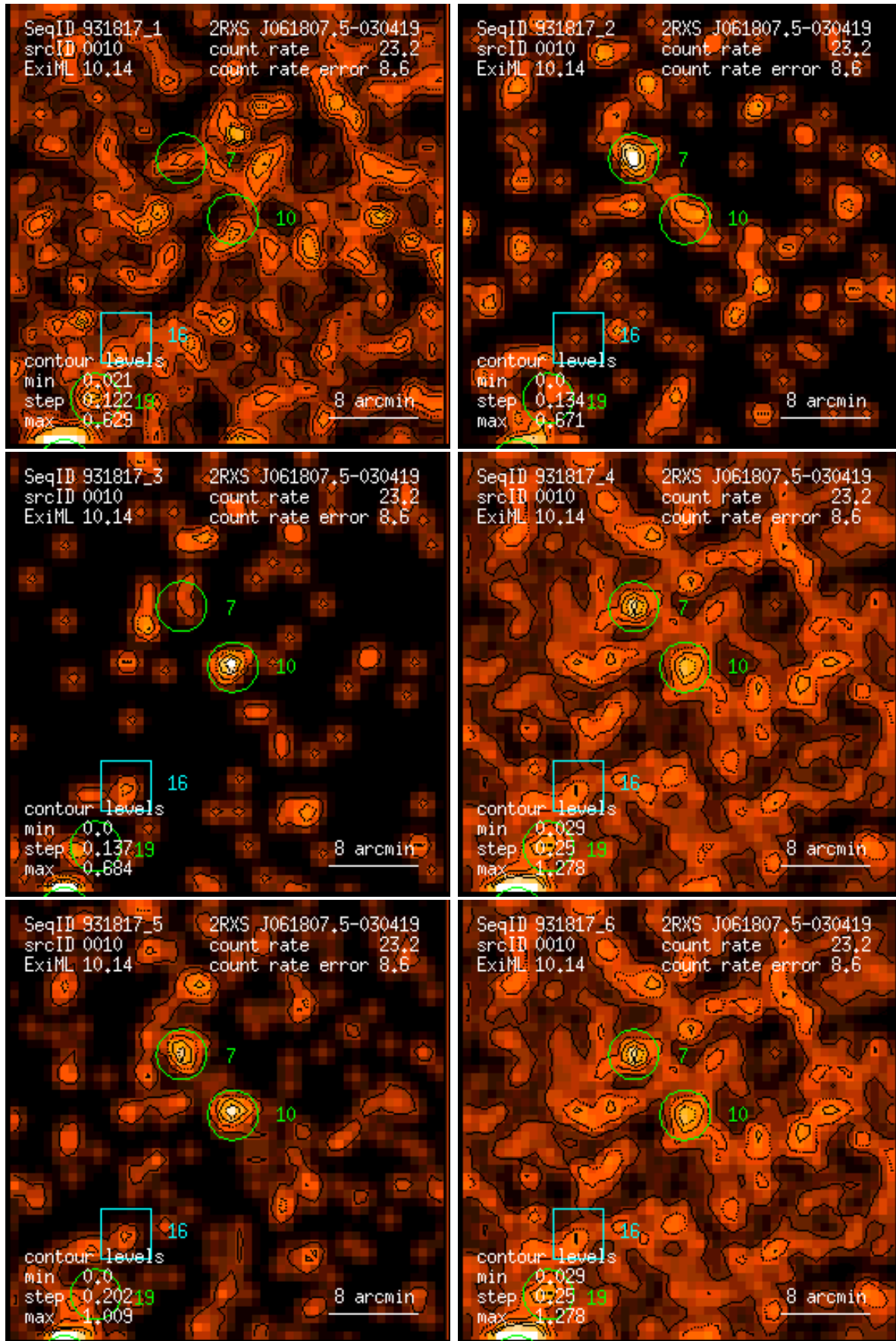
Figure 10: RASS 931817: detection 0010: band rate images, Gaussian filter: (1) PSPC channels 11 – 41, (2) 52 – 90, (3) 91 – 201, (4) 11 – 235, (5) 52 – 201, (6) 11 – 201. Broad band rates in counts/ks. Band rate contour levels in counts/ks/arcmin 2 .
