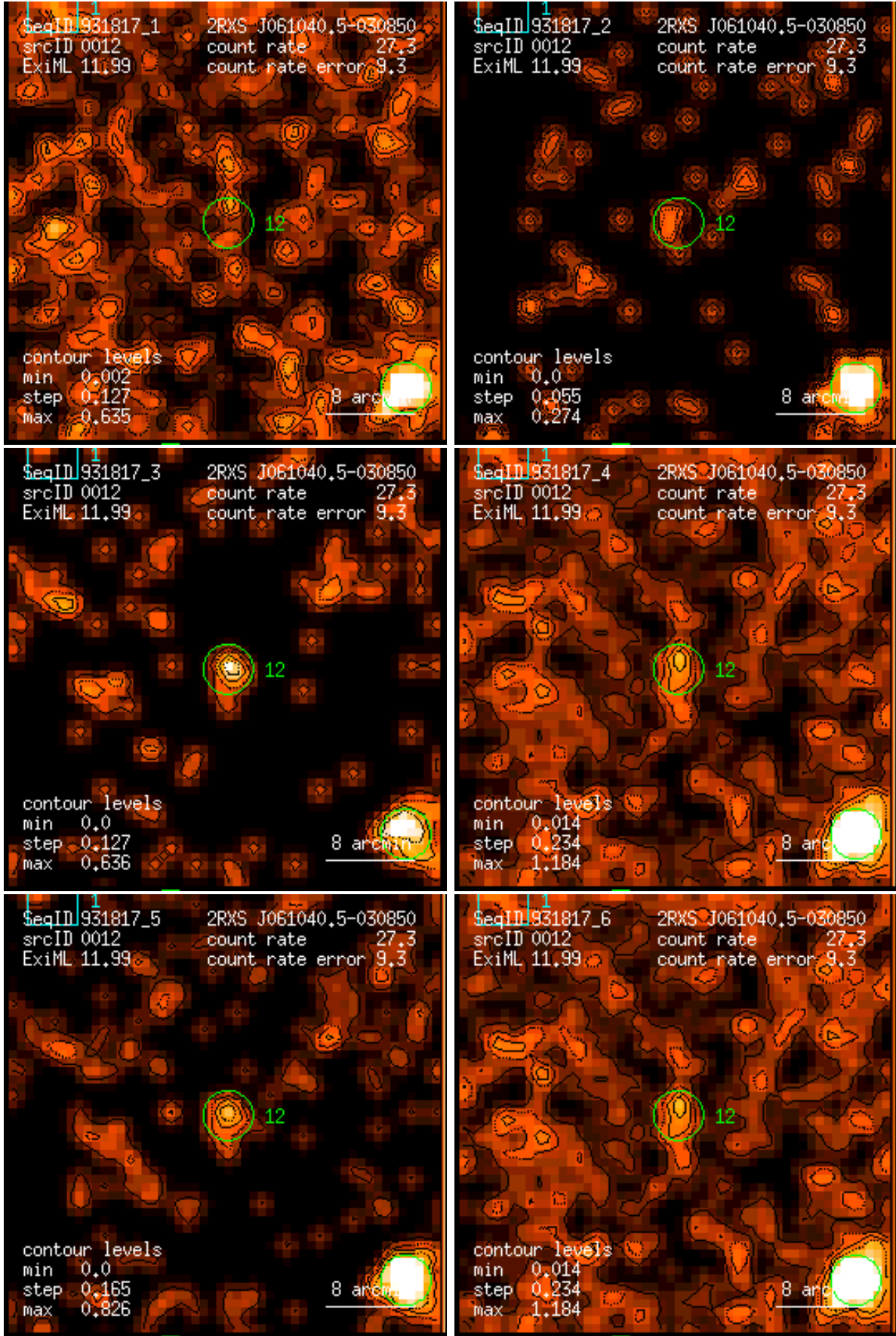
Figure 12: RASS 931817: detection 0012: band rate images, Gaussian filter: (1) PSPC channels 11 – 41, (2) 52 – 90, (3) 91 – 201, (4) 11 – 235, (5) 52 – 201, (6) 11 – 201. Broad band rates in counts/ks. Band rate contour levels in counts/ks/arcmin 2 .
