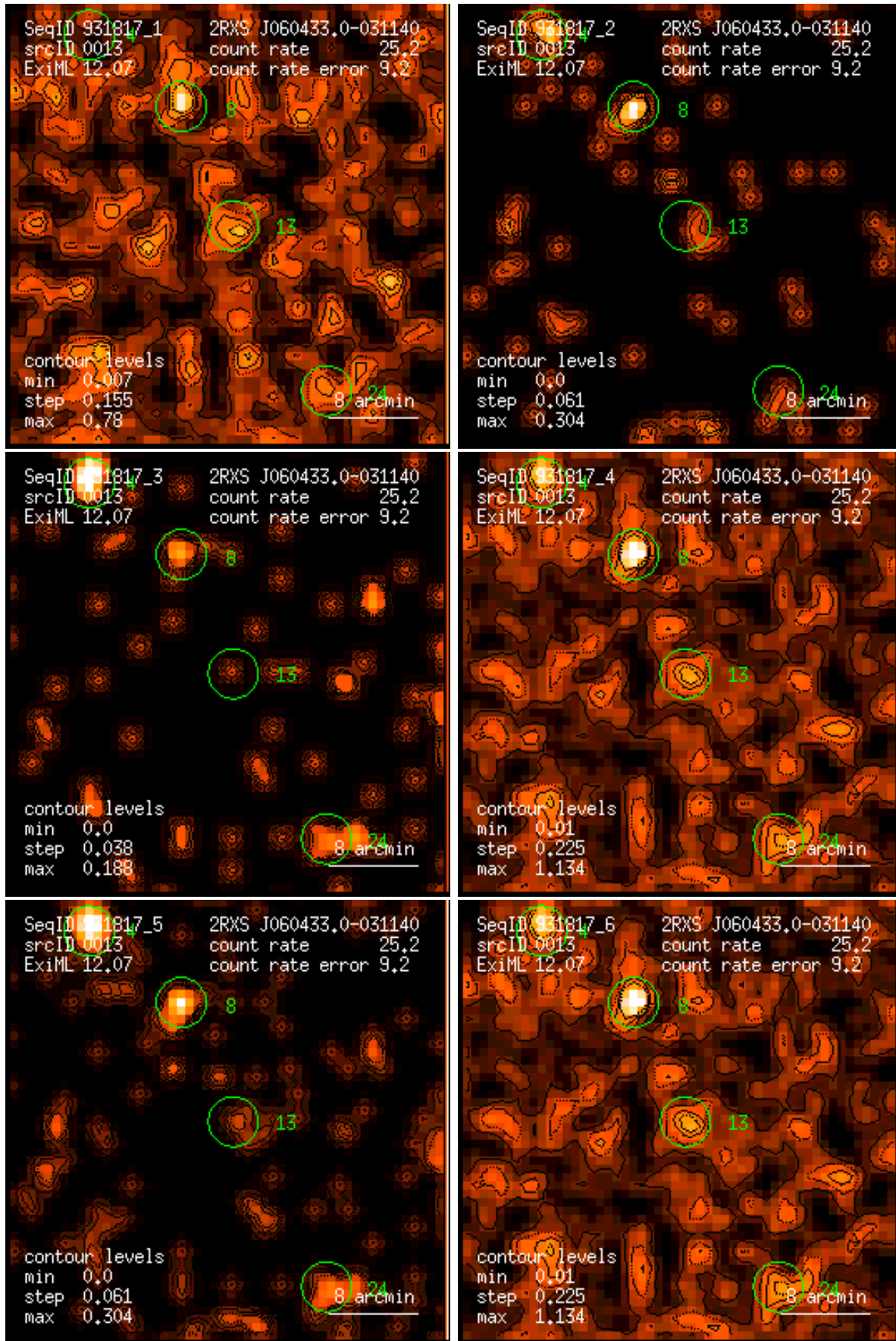
Figure 13: RASS 931817: detection 0013: band rate images, Gaussian filter: (1) PSPC channels 11 – 41, (2) 52 – 90, (3) 91 – 201, (4) 11 – 235, (5) 52 – 201, (6) 11 – 201. Broad band rates in counts/ks. Band rate contour levels in counts/ks/arcmin 2 .
