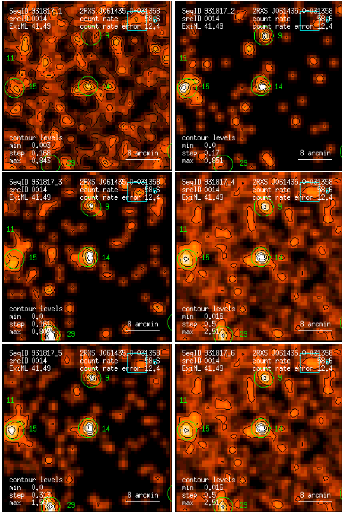
Figure 14: RASS 931817: detection 0014: band rate images, Gaussian filter: (1) PSPC channels 11 – 41, (2) 52 – 90, (3) 91 – 201, (4) 11 – 235, (5) 52 – 201, (6) 11 – 201. Broad band rates in counts/ks. Band rate contour levels in counts/ks/arcmin 2 .
