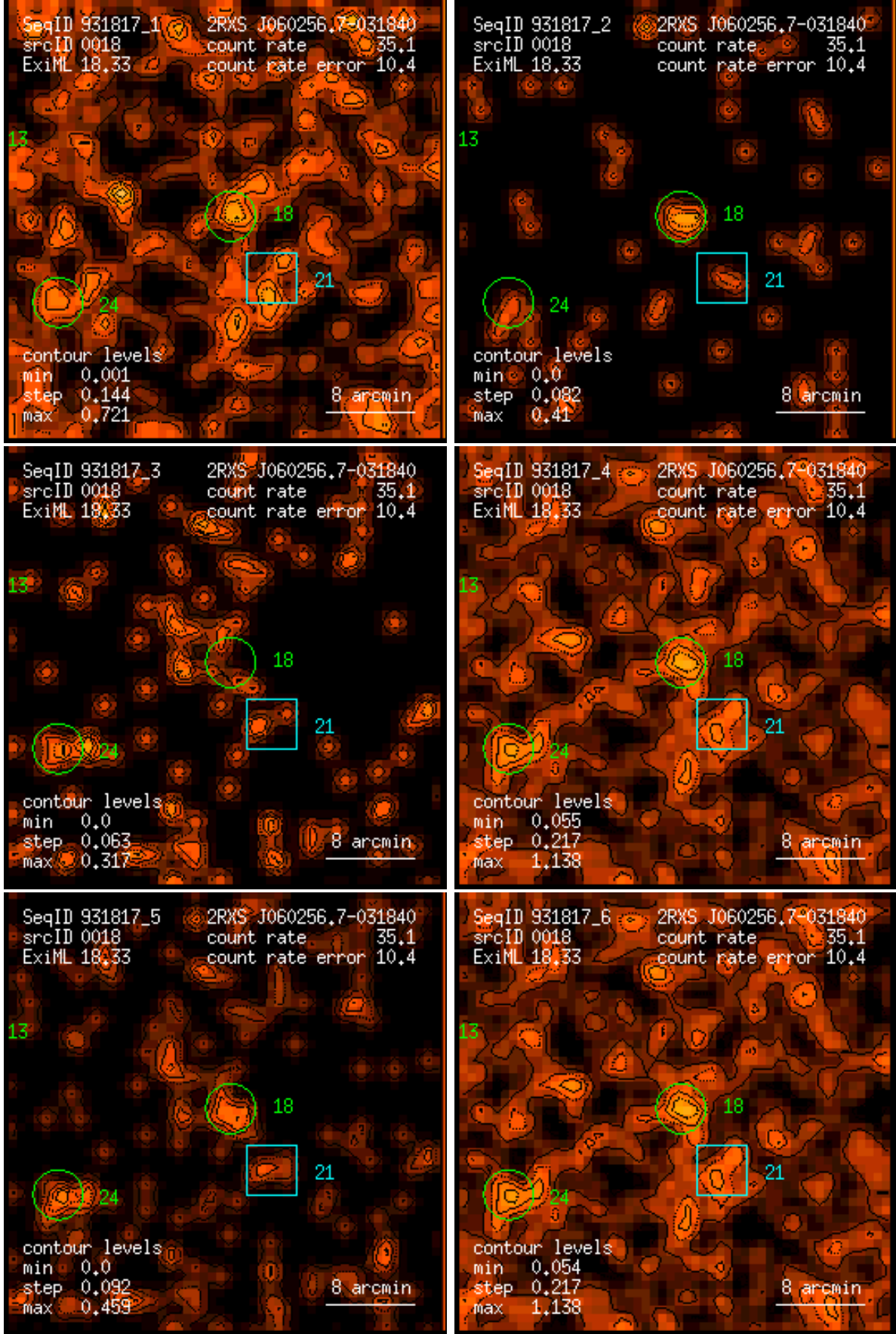
Figure 18: RASS 931817: detection 0018: band rate images, Gaussian filter: (1) PSPC channels 11 – 41, (2) 52 – 90, (3) 91 – 201, (4) 11 – 235, (5) 52 – 201, (6) 11 – 201. Broad band rates in counts/ks. Band rate contour levels in counts/ks/arcmin 2 .
