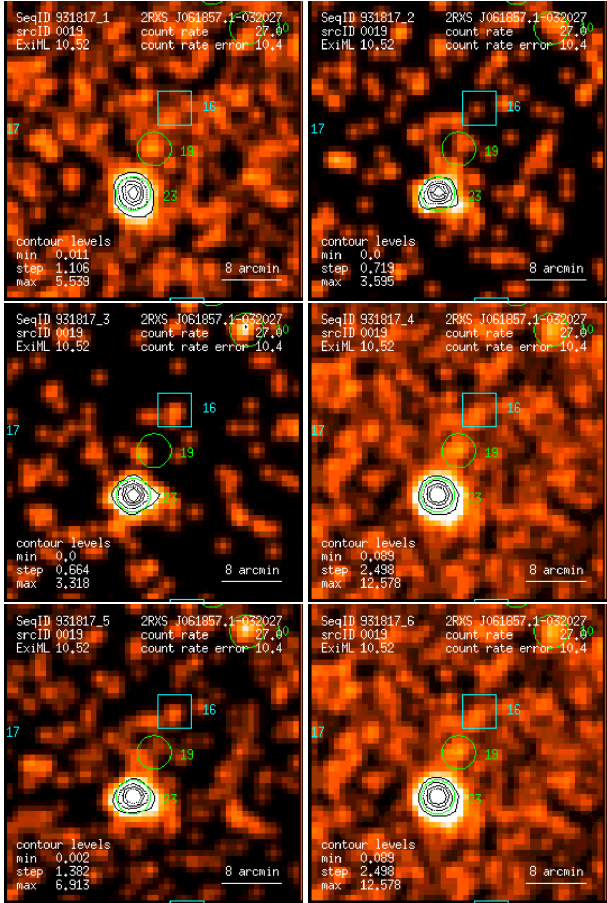
Figure 19: RASS 931817: detection 0019: band rate images, Gaussian filter: (1) PSPC channels 11 – 41, (2) 52 – 90, (3) 91 – 201, (4) 11 – 235, (5) 52 – 201, (6) 11 – 201. Broad band rates in counts/ks. Band rate contour levels in counts/ks/arcmin 2 .
