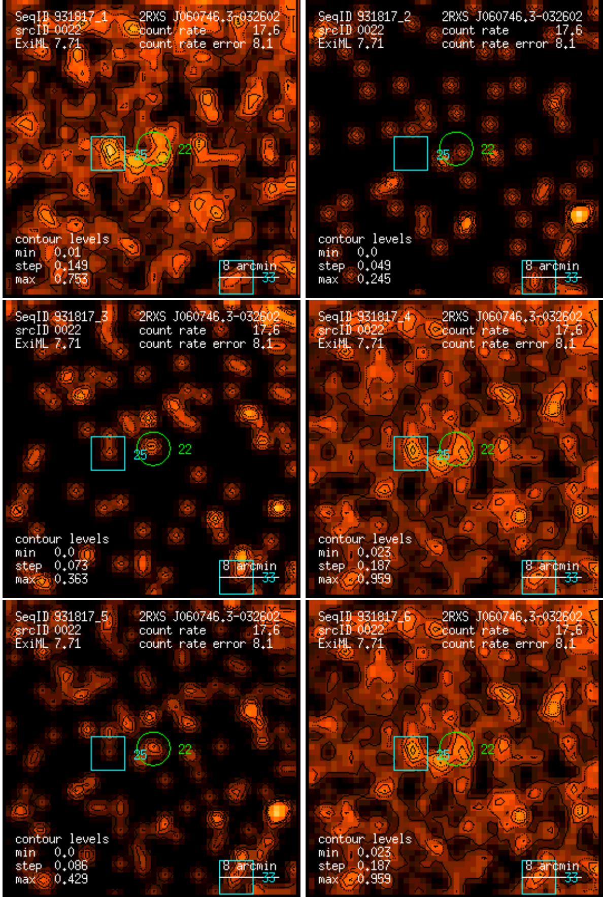
Figure 22: RASS 931817: detection 0022: band rate images, Gaussian filter: (1) PSPC channels 11 – 41, (2) 52 – 90, (3) 91 – 201, (4) 11 – 235, (5) 52 – 201, (6) 11 – 201. Broad band rates in counts/ks. Band rate contour levels in counts/ks/arcmin 2 .
