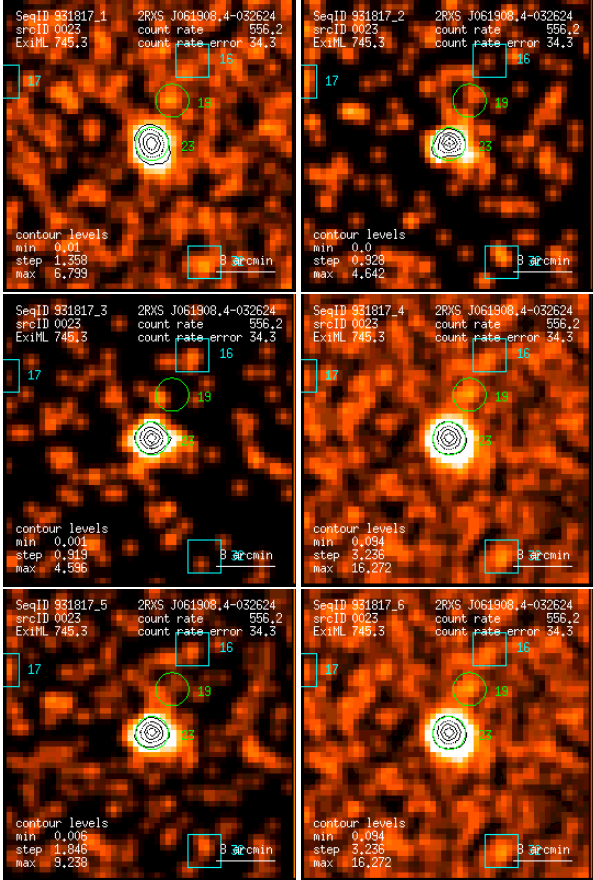
Figure 23: RASS 931817: detection 0023: band rate images, Gaussian filter: (1) PSPC channels 11 – 41, (2) 52 – 90, (3) 91 – 201, (4) 11 – 235, (5) 52 – 201, (6) 11 – 201. Broad band rates in counts/ks. Band rate contour levels in counts/ks/arcmin 2 .
