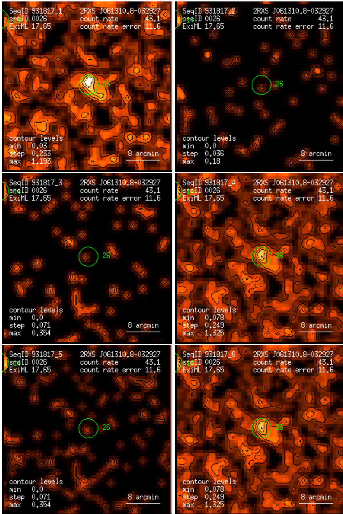
Figure 26: RASS 931817: detection 0026: band rate images, Gaussian filter: (1) PSPC channels 11 – 41, (2) 52 – 90, (3) 91 – 201, (4) 11 – 235, (5) 52 – 201, (6) 11 – 201. Broad band rates in counts/ks. Band rate contour levels in counts/ks/arcmin 2 .
