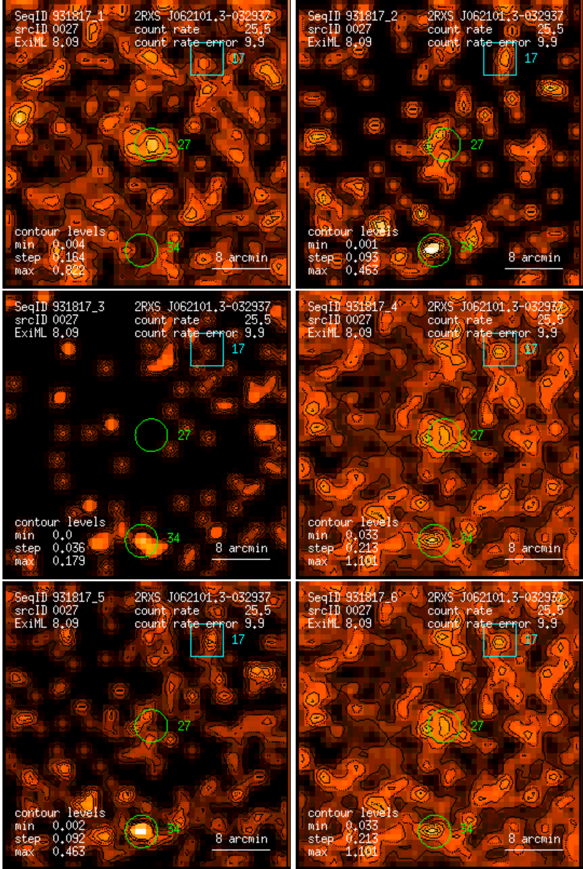
Figure 27: RASS 931817: detection 0027: band rate images, Gaussian filter: (1) PSPC channels 11 – 41, (2) 52 – 90, (3) 91 – 201, (4) 11 – 235, (5) 52 – 201, (6) 11 – 201. Broad band rates in counts/ks. Band rate contour levels in counts/ks/arcmin 2 .
