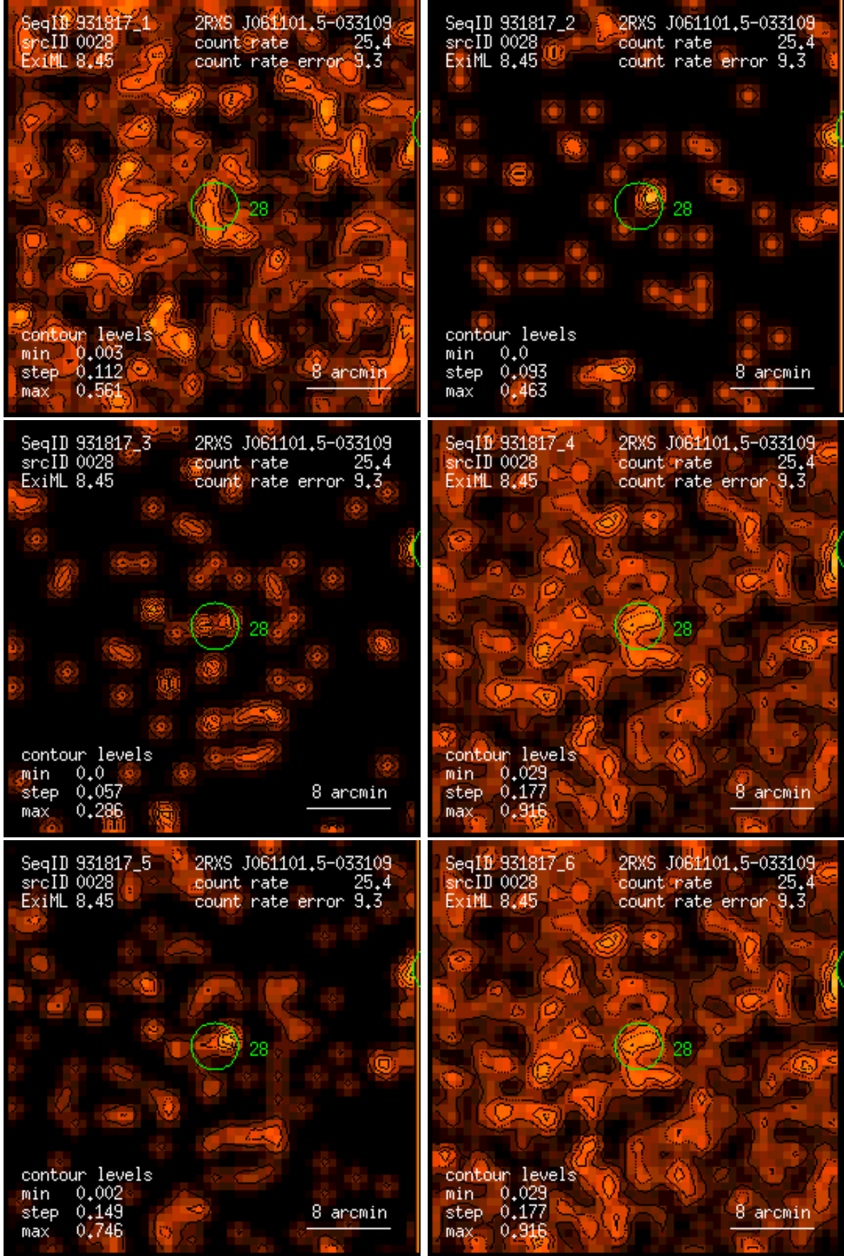
Figure 28: RASS 931817: detection 0028: band rate images, Gaussian filter: (1) PSPC channels 11 – 41, (2) 52 – 90, (3) 91 – 201, (4) 11 – 235, (5) 52 – 201, (6) 11 – 201. Broad band rates in counts/ks. Band rate contour levels in counts/ks/arcmin 2 .
