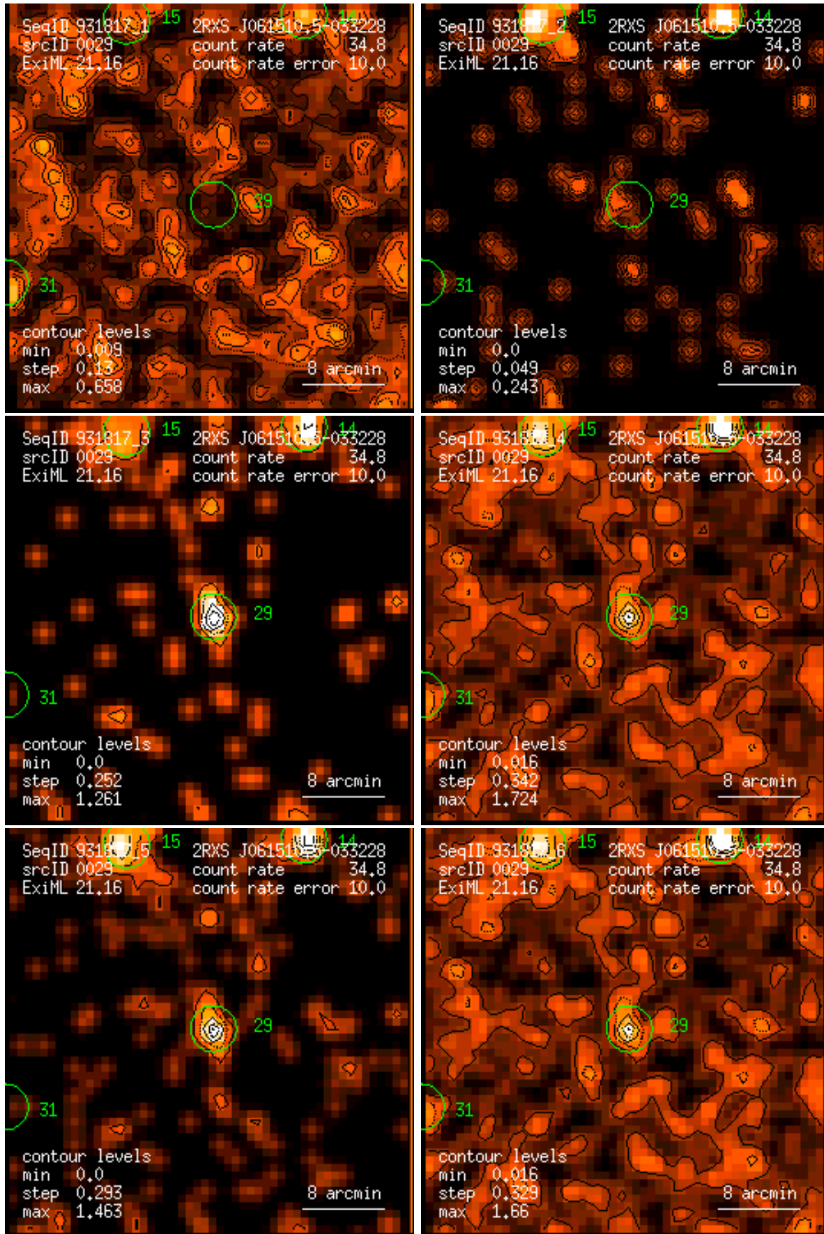
Figure 29: RASS 931817: detection 0029: band rate images, Gaussian filter: (1) PSPC channels 11 – 41, (2) 52 – 90, (3) 91 – 201, (4) 11 – 235, (5) 52 – 201, (6) 11 – 201. Broad band rates in counts/ks. Band rate contour levels in counts/ks/arcmin 2 .
