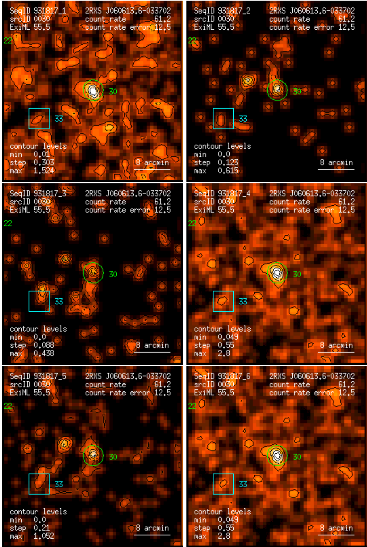
Figure 30: RASS 931817: detection 0030: band rate images, Gaussian filter: (1) PSPC channels 11 – 41, (2) 52 – 90, (3) 91 – 201, (4) 11 – 235, (5) 52 – 201, (6) 11 – 201. Broad band rates in counts/ks. Band rate contour levels in counts/ks/arcmin 2 .
