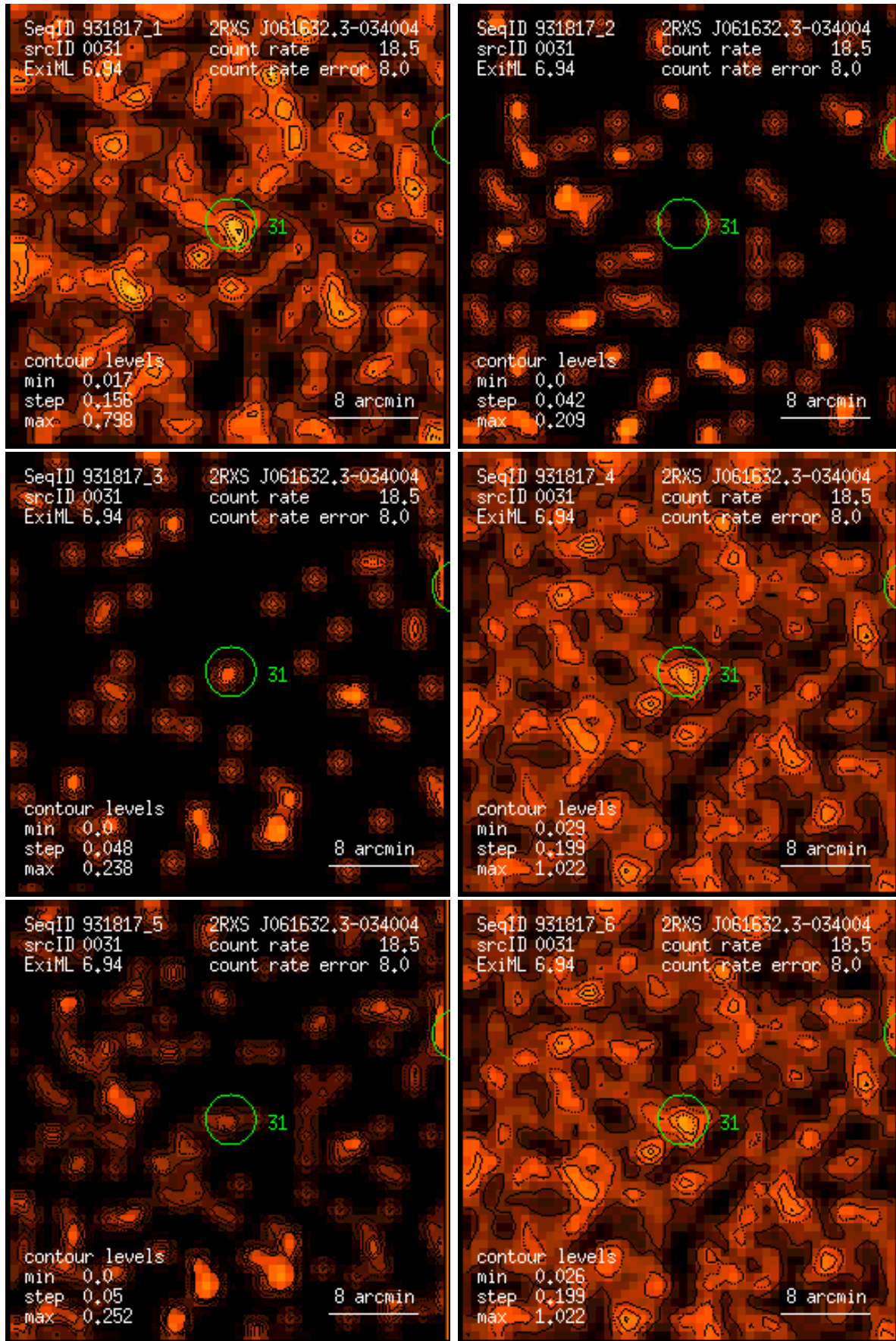
Figure 31: RASS 931817: detection 0031: band rate images, Gaussian filter: (1) PSPC channels 11 – 41, (2) 52 – 90, (3) 91 – 201, (4) 11 – 235, (5) 52 – 201, (6) 11 – 201. Broad band rates in counts/ks. Band rate contour levels in counts/ks/arcmin 2 .
