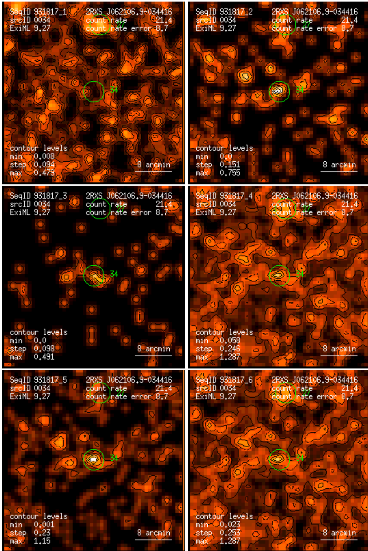
Figure 34: RASS 931817: detection 0034: band rate images, Gaussian filter: (1) PSPC channels 11 – 41, (2) 52 – 90, (3) 91 – 201, (4) 11 – 235, (5) 52 – 201, (6) 11 – 201. Broad band rates in counts/ks. Band rate contour levels in counts/ks/arcmin 2 .
