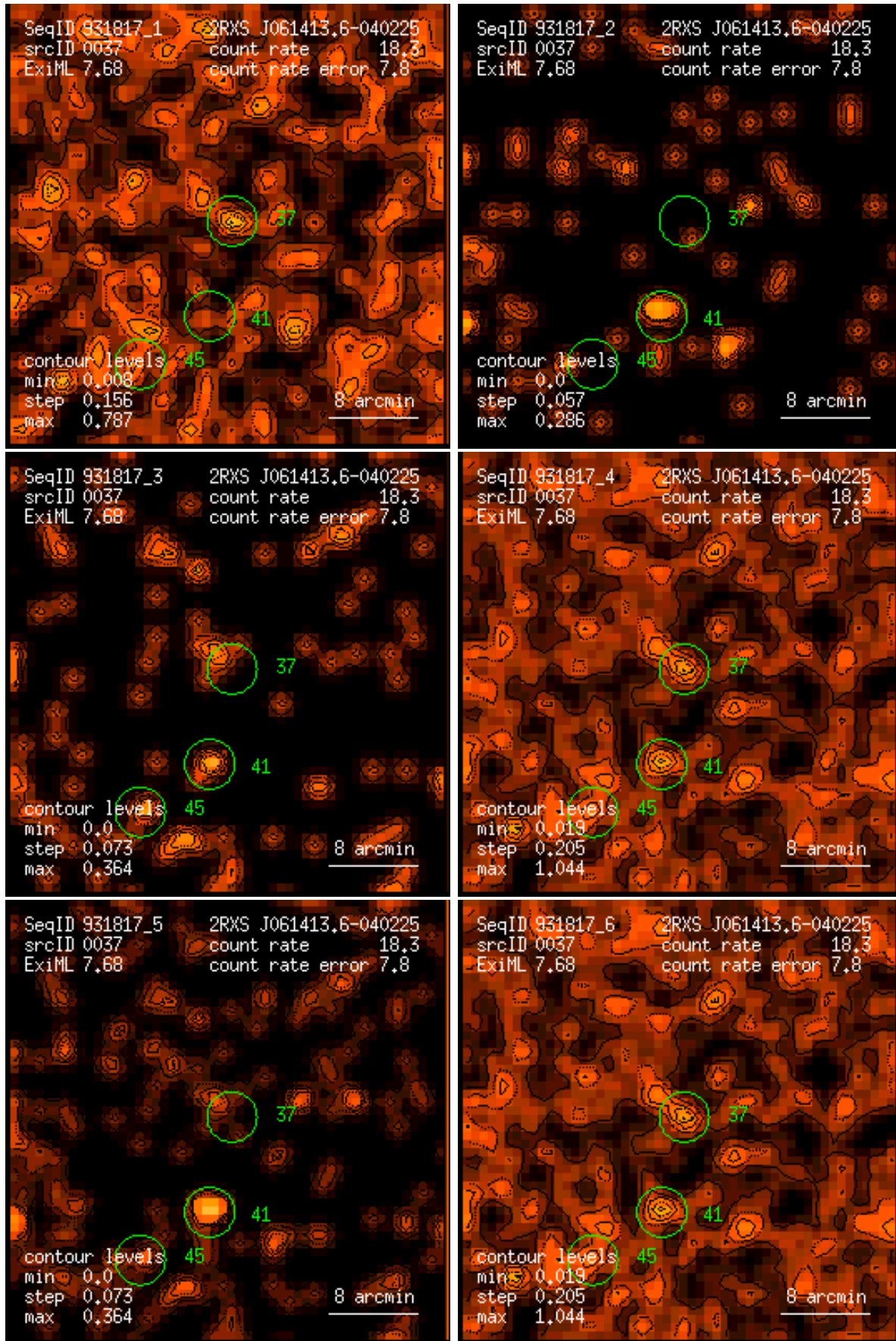
Figure 37: RASS 931817: detection 0037: band rate images, Gaussian filter: (1) PSPC channels 11 – 41, (2) 52 – 90, (3) 91 – 201, (4) 11 – 235, (5) 52 – 201, (6) 11 – 201. Broad band rates in counts/ks. Band rate contour levels in counts/ks/arcmin 2 .
