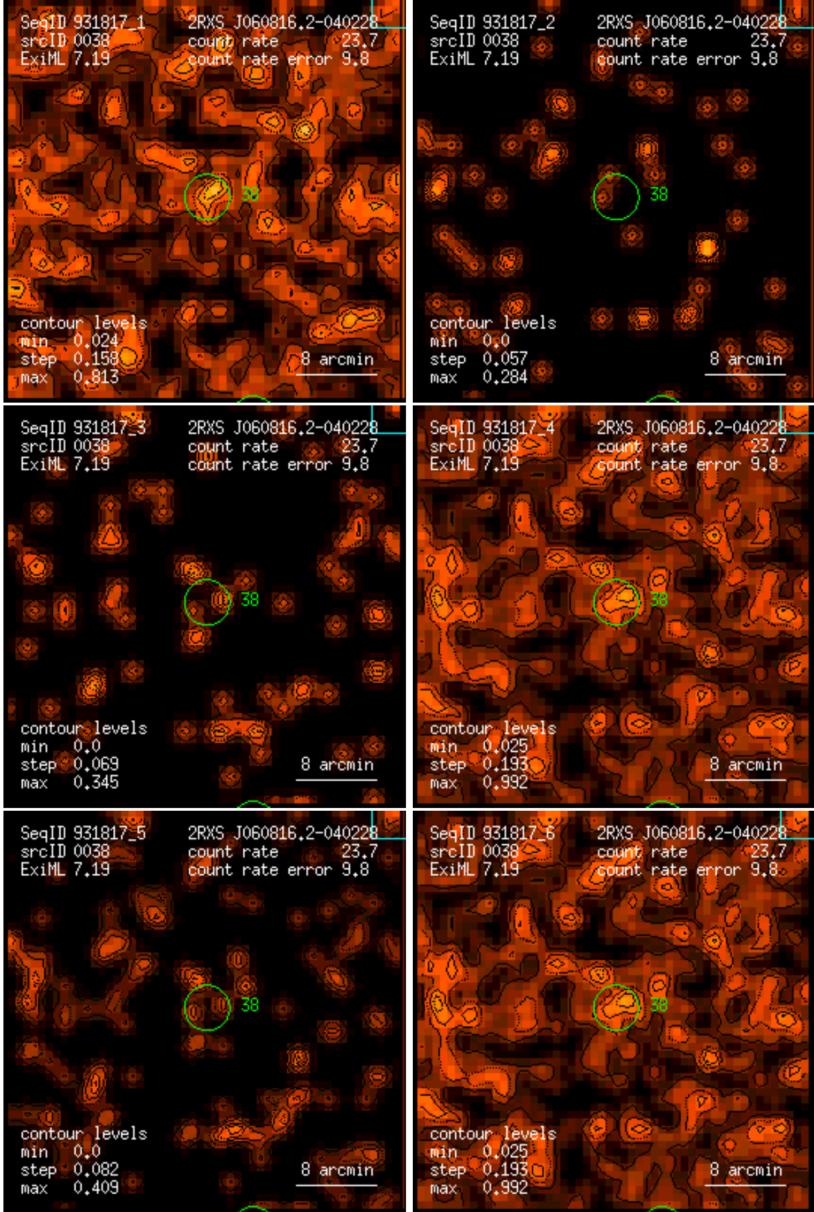
Figure 38: RASS 931817: detection 0038: band rate images, Gaussian filter: (1) PSPC channels 11 – 41, (2) 52 – 90, (3) 91 – 201, (4) 11 – 235, (5) 52 – 201, (6) 11 – 201. Broad band rates in counts/ks. Band rate contour levels in counts/ks/arcmin 2 .
