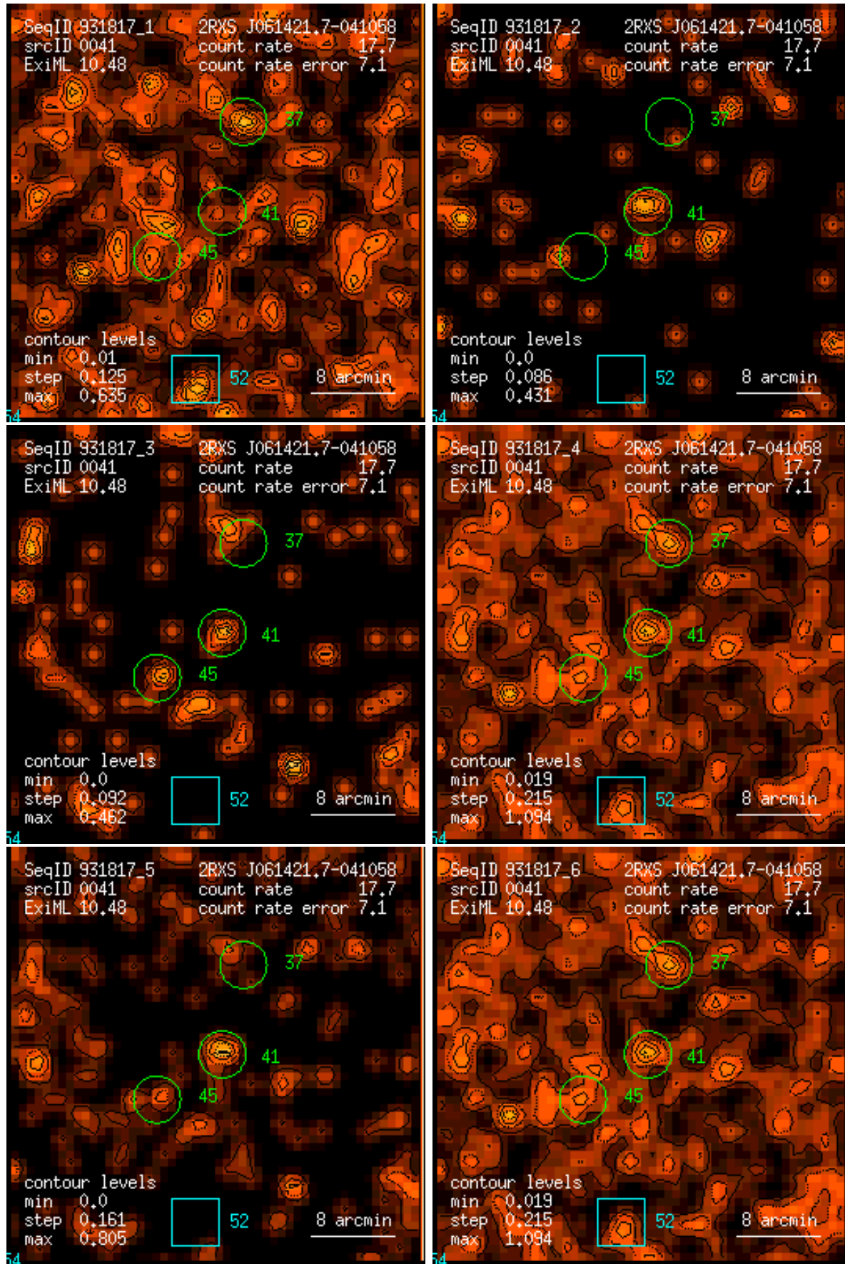
Figure 41: RASS 931817: detection 0041: band rate images, Gaussian filter: (1) PSPC channels 11 – 41, (2) 52 – 90, (3) 91 – 201, (4) 11 – 235, (5) 52 – 201, (6) 11 – 201. Broad band rates in counts/ks. Band rate contour levels in counts/ks/arcmin 2 .
