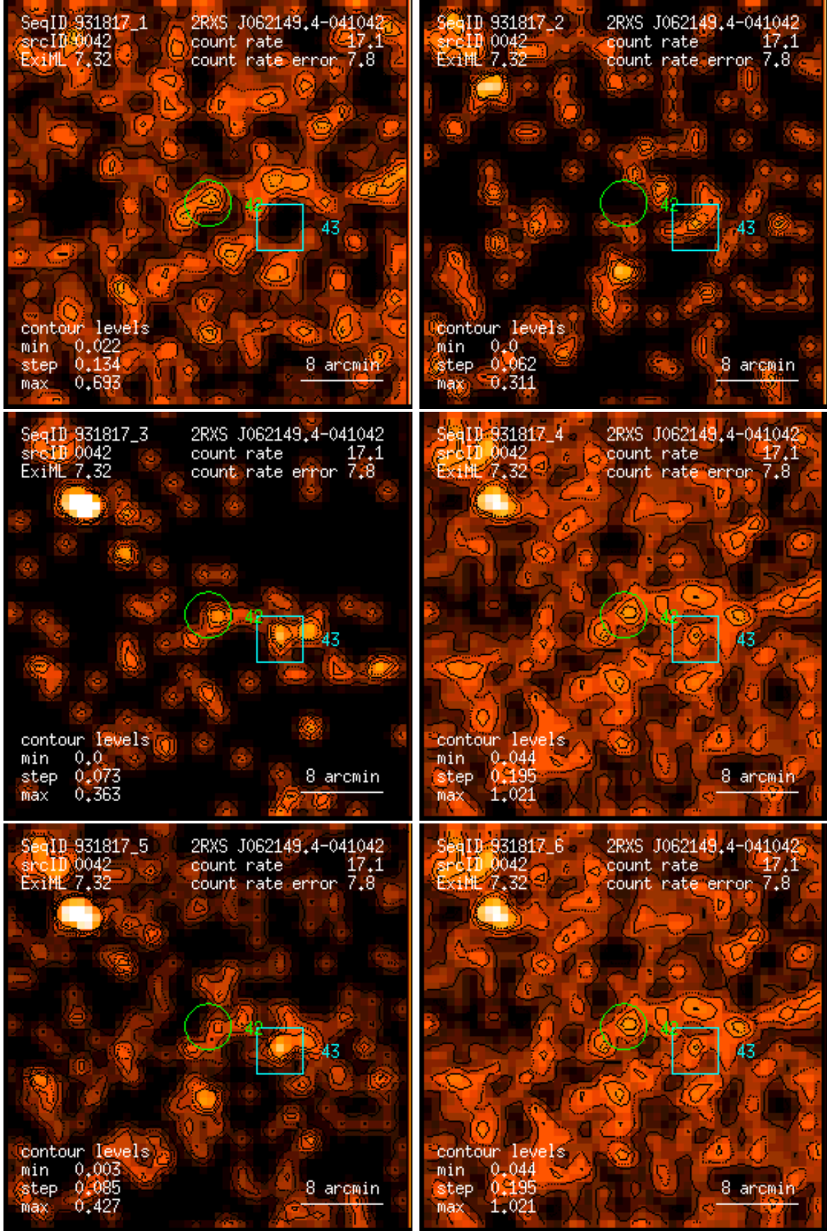
Figure 42: RASS 931817: detection 0042: band rate images, Gaussian filter: (1) PSPC channels 11 – 41, (2) 52 – 90, (3) 91 – 201, (4) 11 – 235, (5) 52 – 201, (6) 11 – 201. Broad band rates in counts/ks. Band rate contour levels in counts/ks/arcmin 2 .
