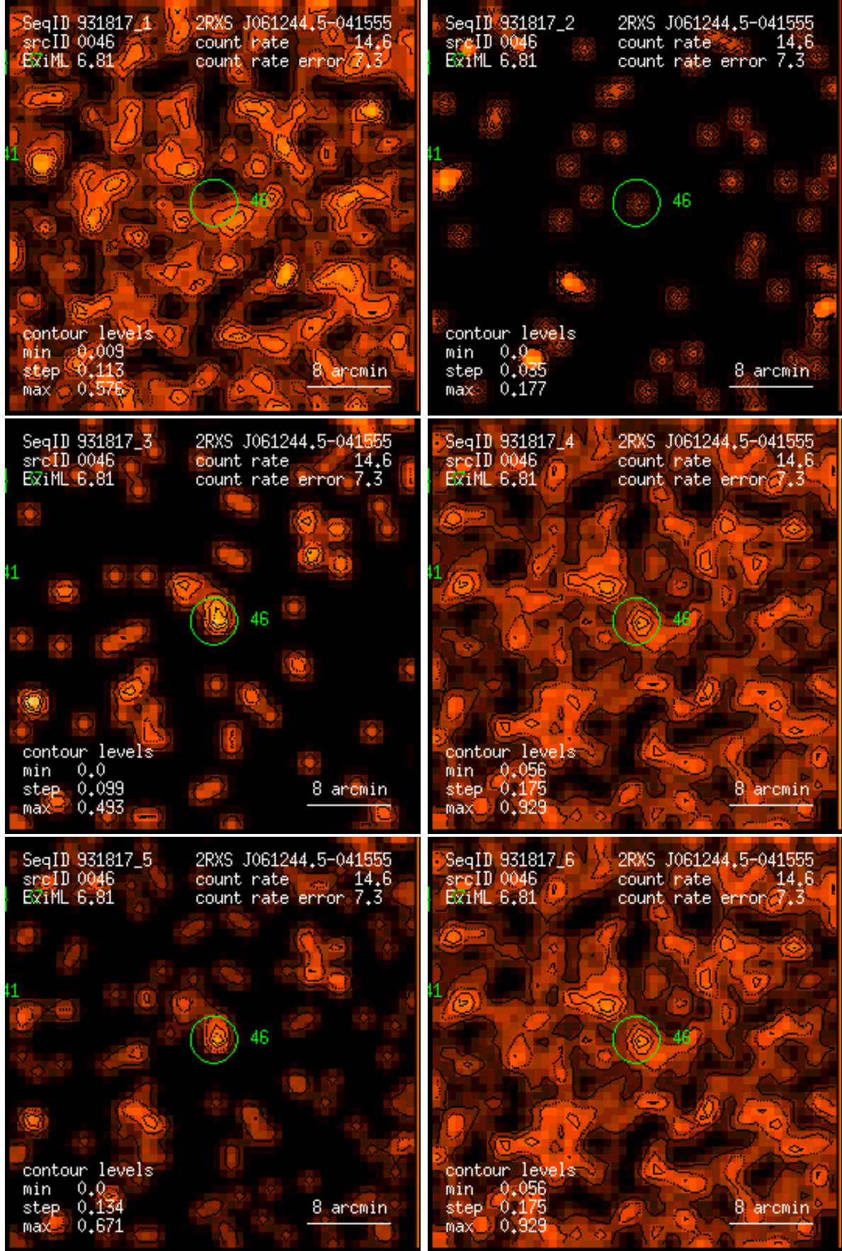
Figure 46: RASS 931817: detection 0046: band rate images, Gaussian filter: (1) PSPC channels 11 – 41, (2) 52 – 90, (3) 91 – 201, (4) 11 – 235, (5) 52 – 201, (6) 11 – 201. Broad band rates in counts/ks. Band rate contour levels in counts/ks/arcmin 2 .
