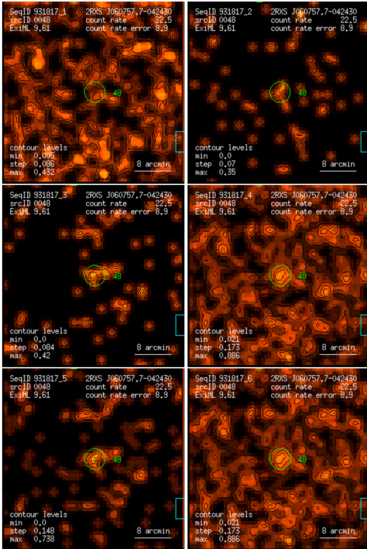
Figure 48: RASS 931817: detection 0048: band rate images, Gaussian filter: (1) PSPC channels 11 – 41, (2) 52 – 90, (3) 91 – 201, (4) 11 – 235, (5) 52 – 201, (6) 11 – 201. Broad band rates in counts/ks. Band rate contour levels in counts/ks/arcmin 2 .
