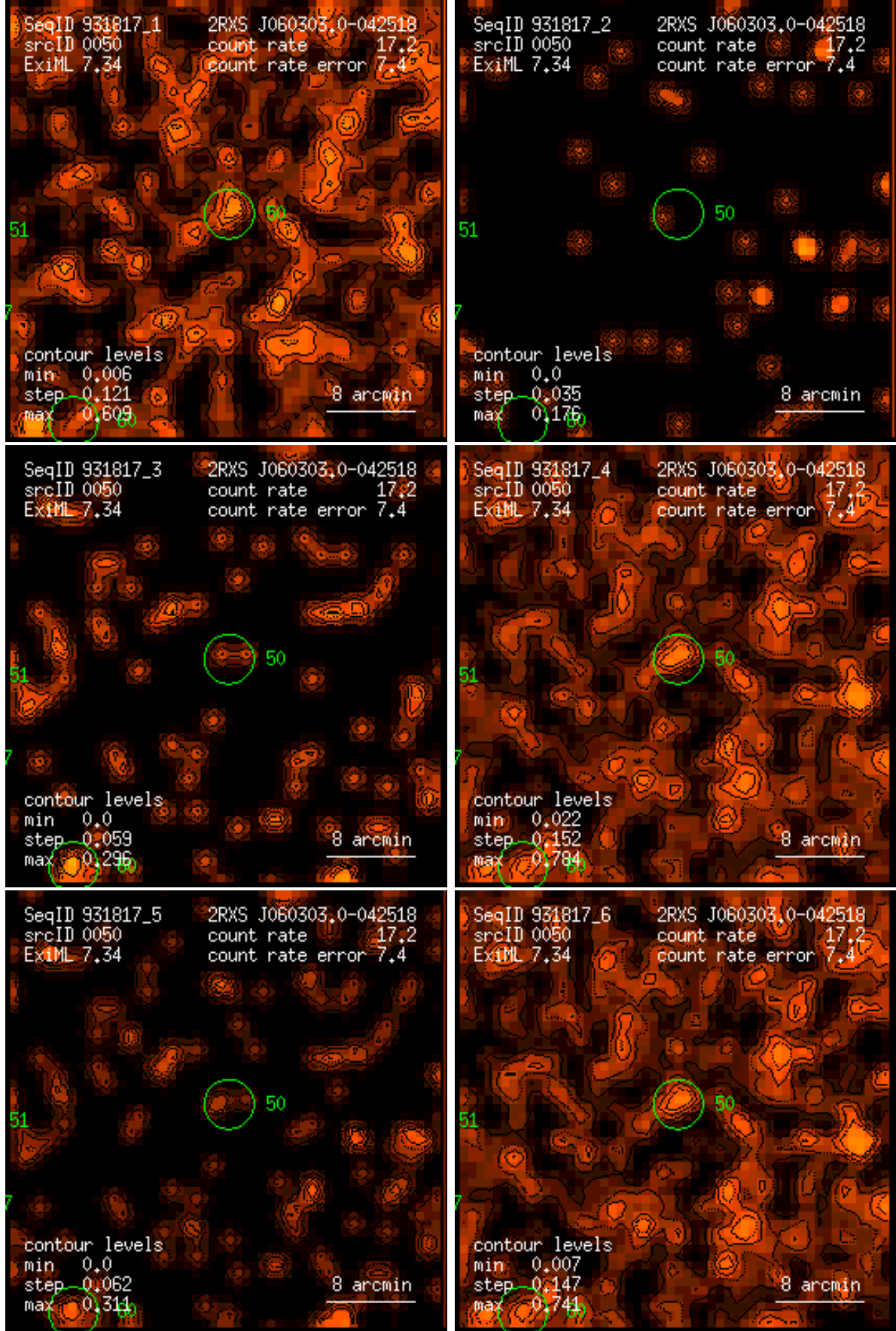
Figure 50: RASS 931817: detection 0050: band rate images, Gaussian filter: (1) PSPC channels 11 – 41, (2) 52 – 90, (3) 91 – 201, (4) 11 – 235, (5) 52 – 201, (6) 11 – 201. Broad band rates in counts/ks. Band rate contour levels in counts/ks/arcmin 2 .
