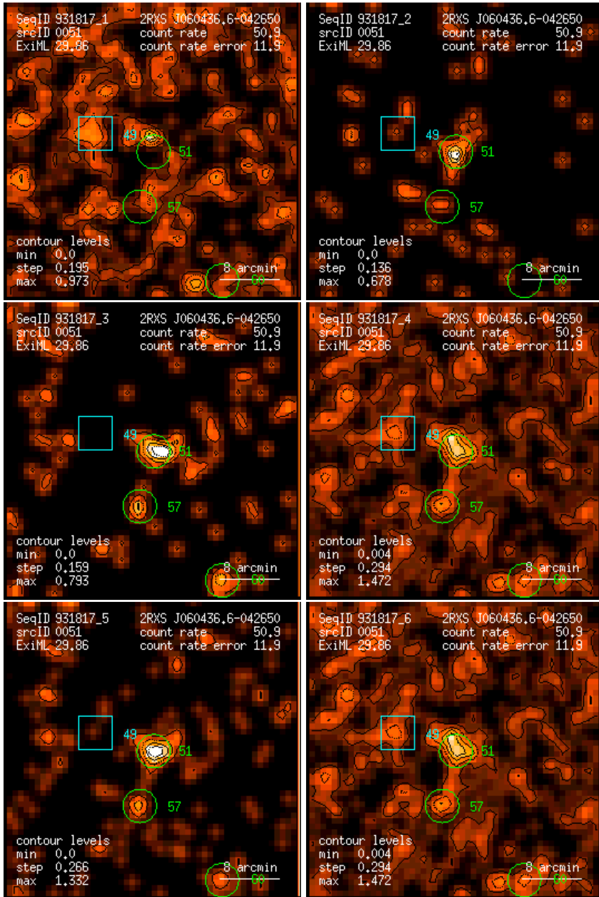
Figure 51: RASS 931817: detection 0051: band rate images, Gaussian filter: (1) PSPC channels 11 – 41, (2) 52 – 90, (3) 91 – 201, (4) 11 – 235, (5) 52 – 201, (6) 11 – 201. Broad band rates in counts/ks. Band rate contour levels in counts/ks/arcmin 2 .
