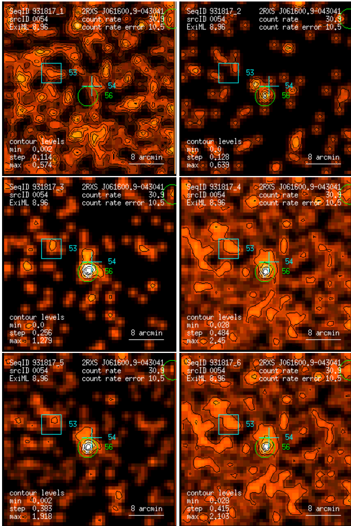
Figure 54: RASS 931817: detection 0054: band rate images, Gaussian filter: (1) PSPC channels 11 – 41, (2) 52 – 90, (3) 91 – 201, (4) 11 – 235, (5) 52 – 201, (6) 11 – 201. Broad band rates in counts/ks. Band rate contour levels in counts/ks/arcmin 2 .
