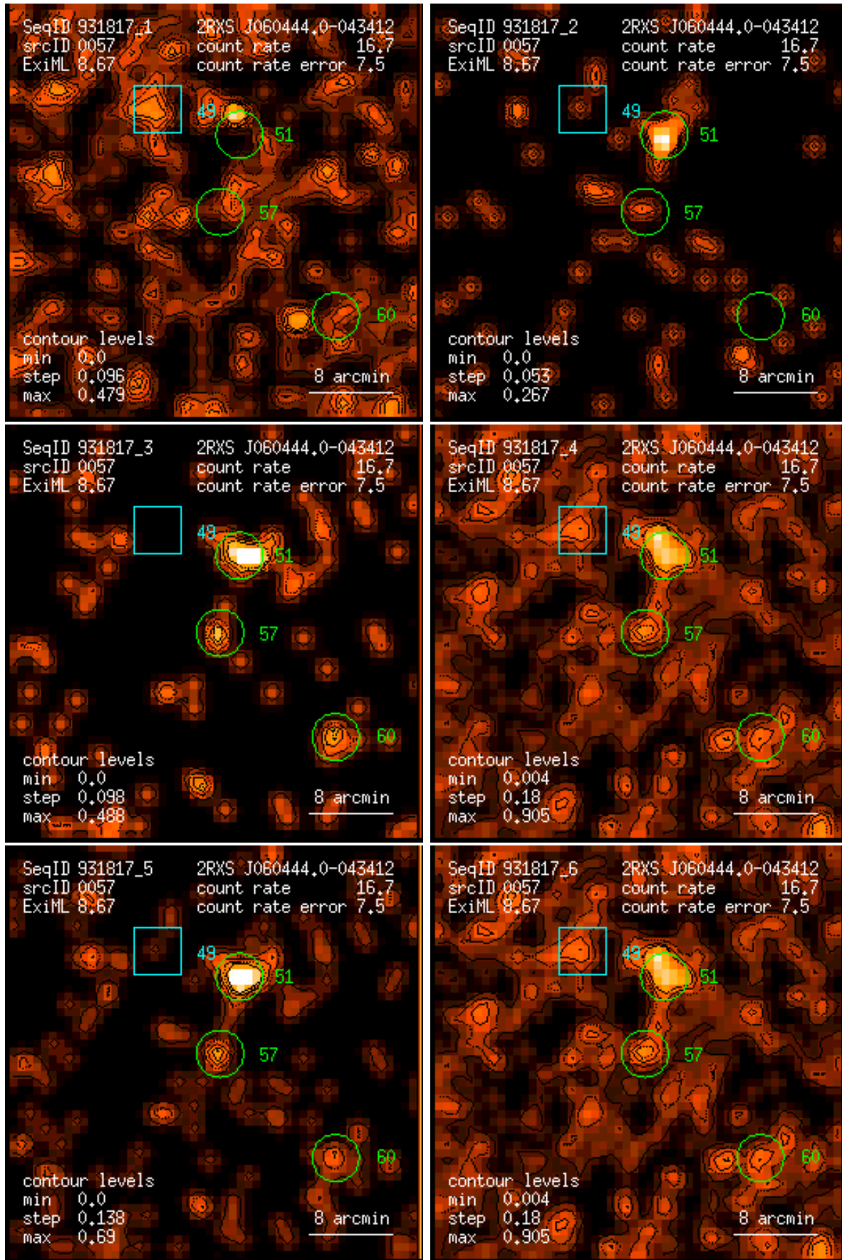
Figure 57: RASS 931817: detection 0057: band rate images, Gaussian filter: (1) PSPC channels 11 – 41, (2) 52 – 90, (3) 91 – 201, (4) 11 – 235, (5) 52 – 201, (6) 11 – 201. Broad band rates in counts/ks. Band rate contour levels in counts/ks/arcmin 2 .
