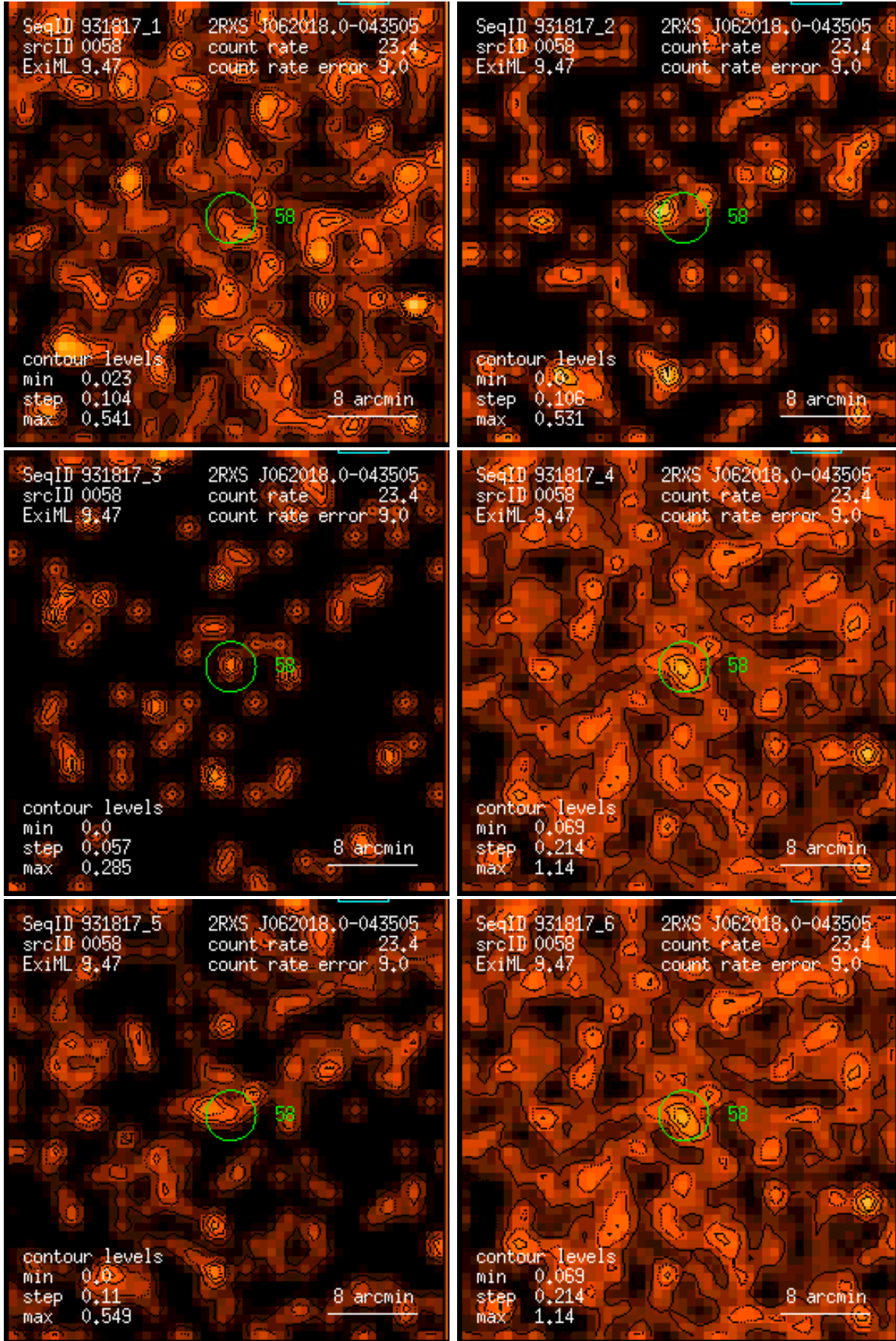
Figure 58: RASS 931817: detection 0058: band rate images, Gaussian filter: (1) PSPC channels 11 – 41, (2) 52 – 90, (3) 91 – 201, (4) 11 – 235, (5) 52 – 201, (6) 11 – 201. Broad band rates in counts/ks. Band rate contour levels in counts/ks/arcmin 2 .
