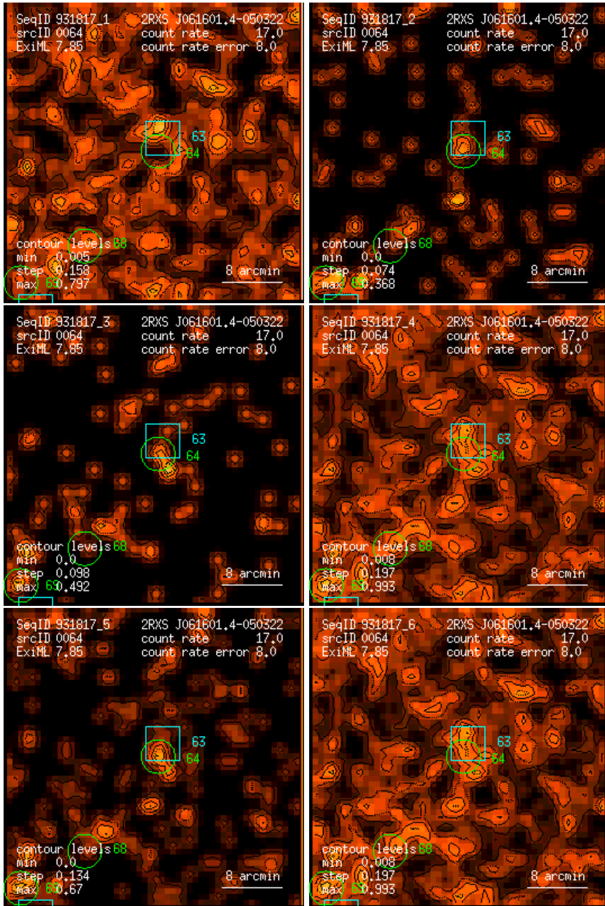
Figure 64: RASS 931817: detection 0064: band rate images, Gaussian filter: (1) PSPC channels 11 – 41, (2) 52 – 90, (3) 91 – 201, (4) 11 – 235, (5) 52 – 201, (6) 11 – 201. Broad band rates in counts/ks. Band rate contour levels in counts/ks/arcmin 2 .
