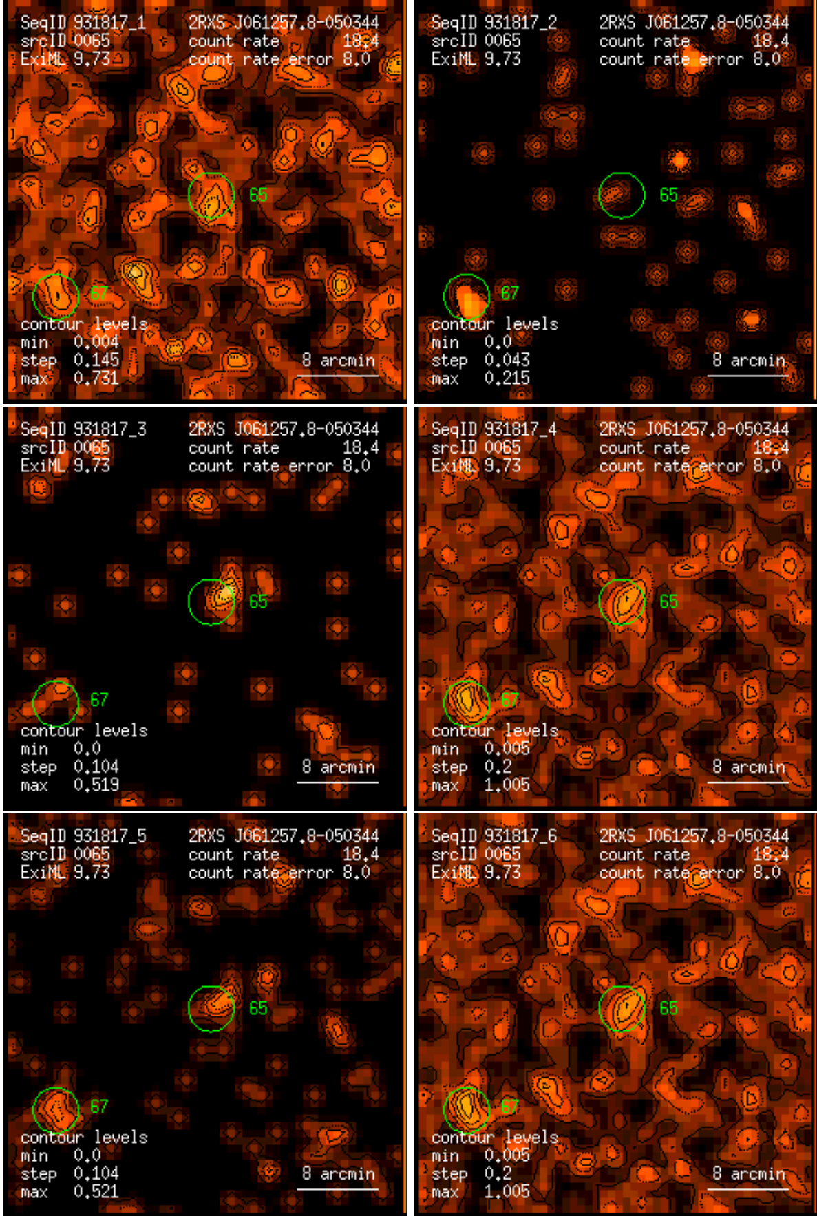
Figure 65: RASS 931817: detection 0065: band rate images, Gaussian filter: (1) PSPC channels 11 – 41, (2) 52 – 90, (3) 91 – 201, (4) 11 – 235, (5) 52 – 201, (6) 11 – 201. Broad band rates in counts/ks. Band rate contour levels in counts/ks/arcmin 2 .
