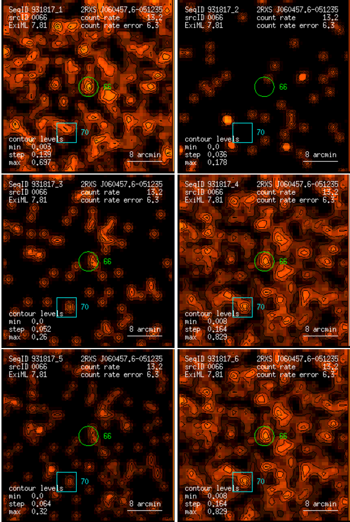
Figure 66: RASS 931817: detection 0066: band rate images, Gaussian filter: (1) PSPC channels 11 – 41, (2) 52 – 90, (3) 91 – 201, (4) 11 – 235, (5) 52 – 201, (6) 11 – 201. Broad band rates in counts/ks. Band rate contour levels in counts/ks/arcmin 2 .
