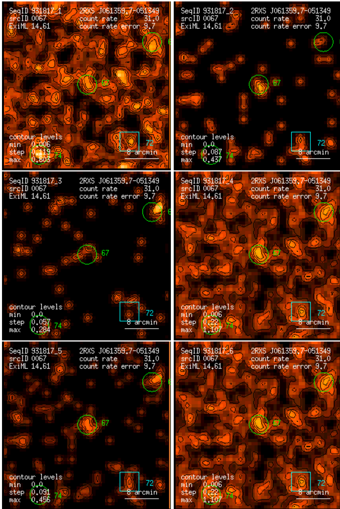
Figure 67: RASS 931817: detection 0067: band rate images, Gaussian filter: (1) PSPC channels 11 – 41, (2) 52 – 90, (3) 91 – 201, (4) 11 – 235, (5) 52 – 201, (6) 11 – 201. Broad band rates in counts/ks. Band rate contour levels in counts/ks/arcmin 2 .
