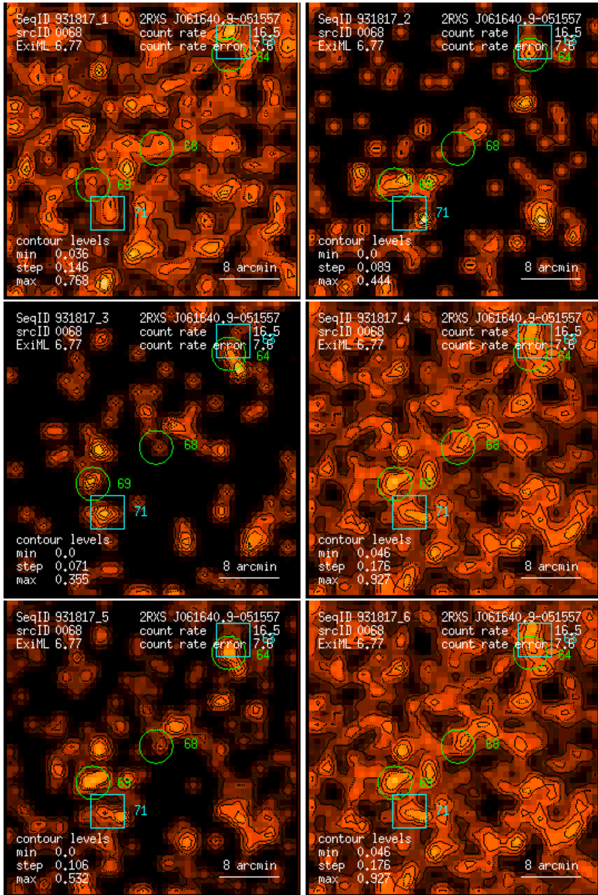
Figure 68: RASS 931817: detection 0068: band rate images, Gaussian filter: (1) PSPC channels 11 – 41, (2) 52 – 90, (3) 91 – 201, (4) 11 – 235, (5) 52 – 201, (6) 11 – 201. Broad band rates in counts/ks. Band rate contour levels in counts/ks/arcmin 2 .
