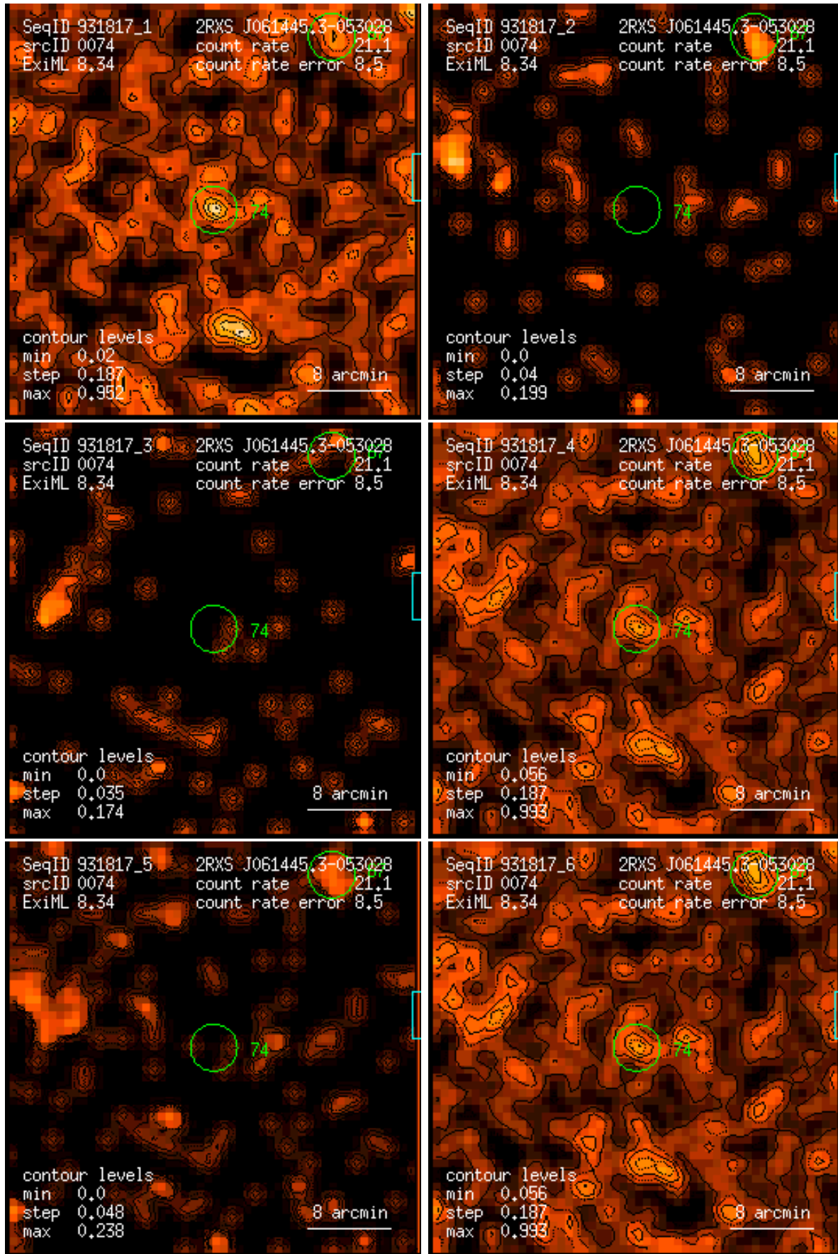
Figure 74: RASS 931817: detection 0074: band rate images, Gaussian filter: (1) PSPC channels 11 – 41, (2) 52 – 90, (3) 91 – 201, (4) 11 – 235, (5) 52 – 201, (6) 11 – 201. Broad band rates in counts/ks. Band rate contour levels in counts/ks/arcmin 2 .
