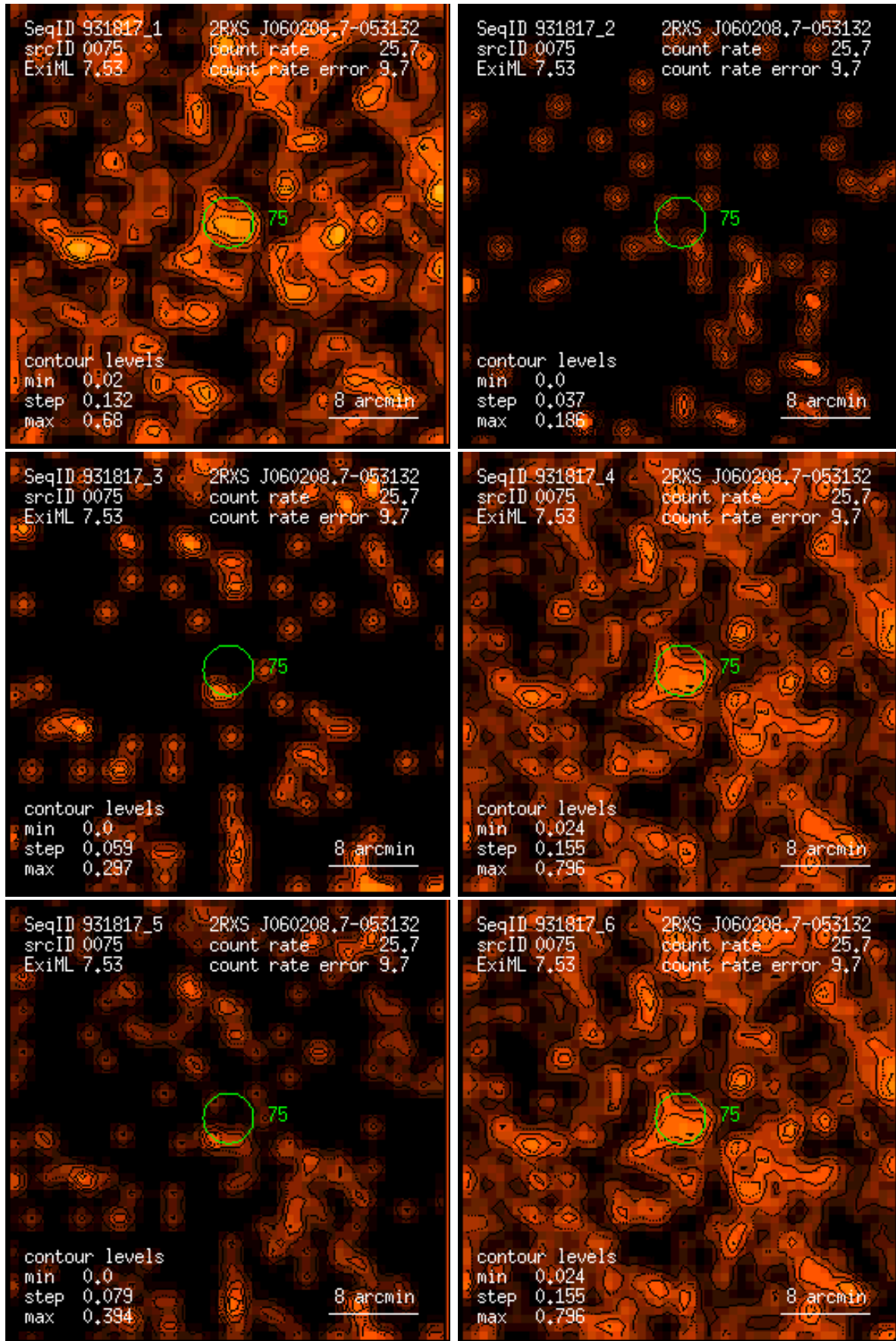
Figure 75: RASS 931817: detection 0075: band rate images, Gaussian filter: (1) PSPC channels 11 – 41, (2) 52 – 90, (3) 91 – 201, (4) 11 – 235, (5) 52 – 201, (6) 11 – 201. Broad band rates in counts/ks. Band rate contour levels in counts/ks/arcmin 2 .
