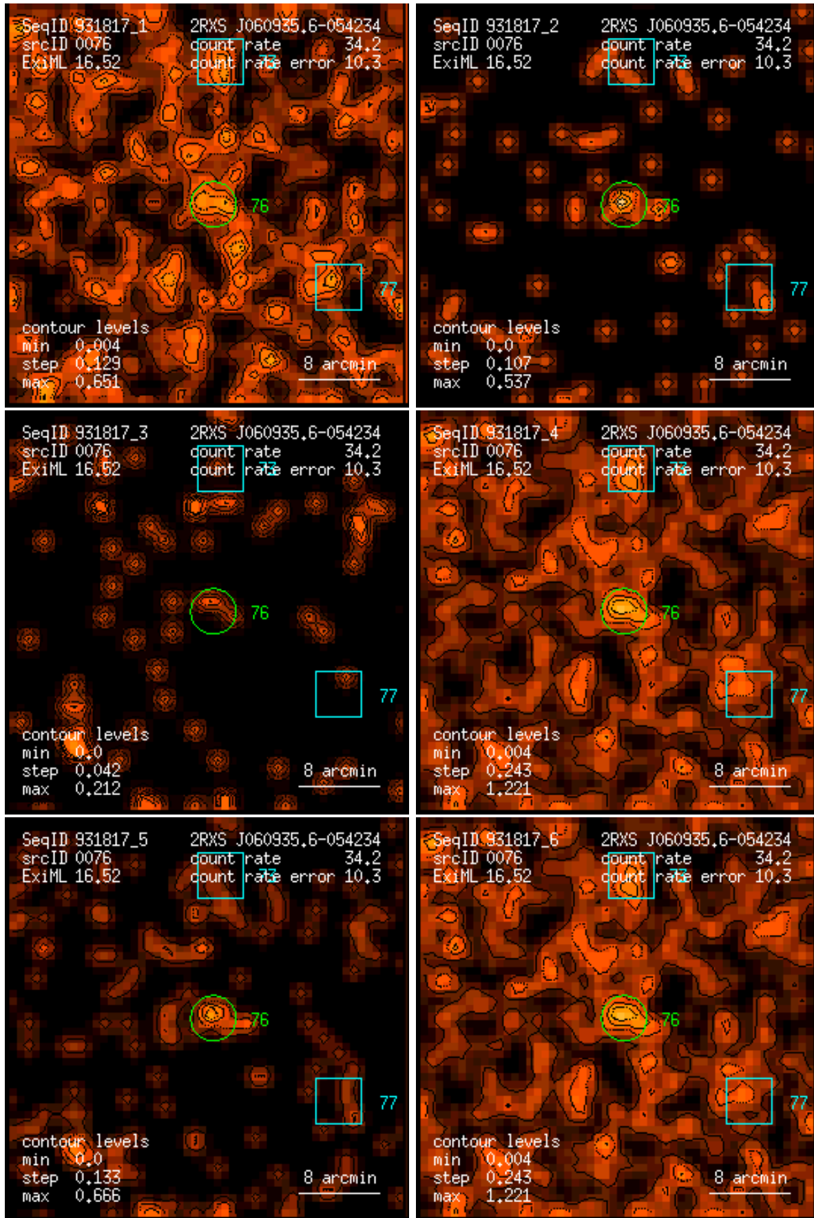
Figure 76: RASS 931817: detection 0076: band rate images, Gaussian filter: (1) PSPC channels 11 – 41, (2) 52 – 90, (3) 91 – 201, (4) 11 – 235, (5) 52 – 201, (6) 11 – 201. Broad band rates in counts/ks. Band rate contour levels in counts/ks/arcmin 2 .
