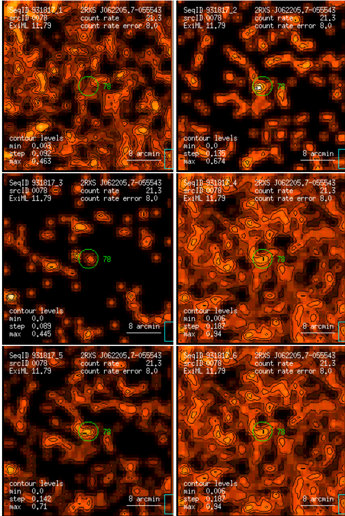
Figure 78: RASS 931817: detection 0078: band rate images, Gaussian filter: (1) PSPC channels 11 – 41, (2) 52 – 90, (3) 91 – 201, (4) 11 – 235, (5) 52 – 201, (6) 11 – 201. Broad band rates in counts/ks. Band rate contour levels in counts/ks/arcmin 2 .
