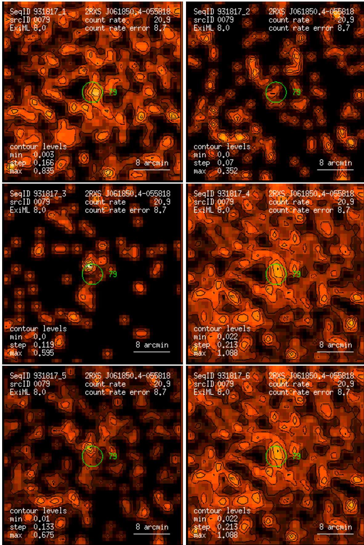
Figure 79: RASS 931817: detection 0079: band rate images, Gaussian filter: (1) PSPC channels 11 – 41, (2) 52 – 90, (3) 91 – 201, (4) 11 – 235, (5) 52 – 201, (6) 11 – 201. Broad band rates in counts/ks. Band rate contour levels in counts/ks/arcmin 2 .
