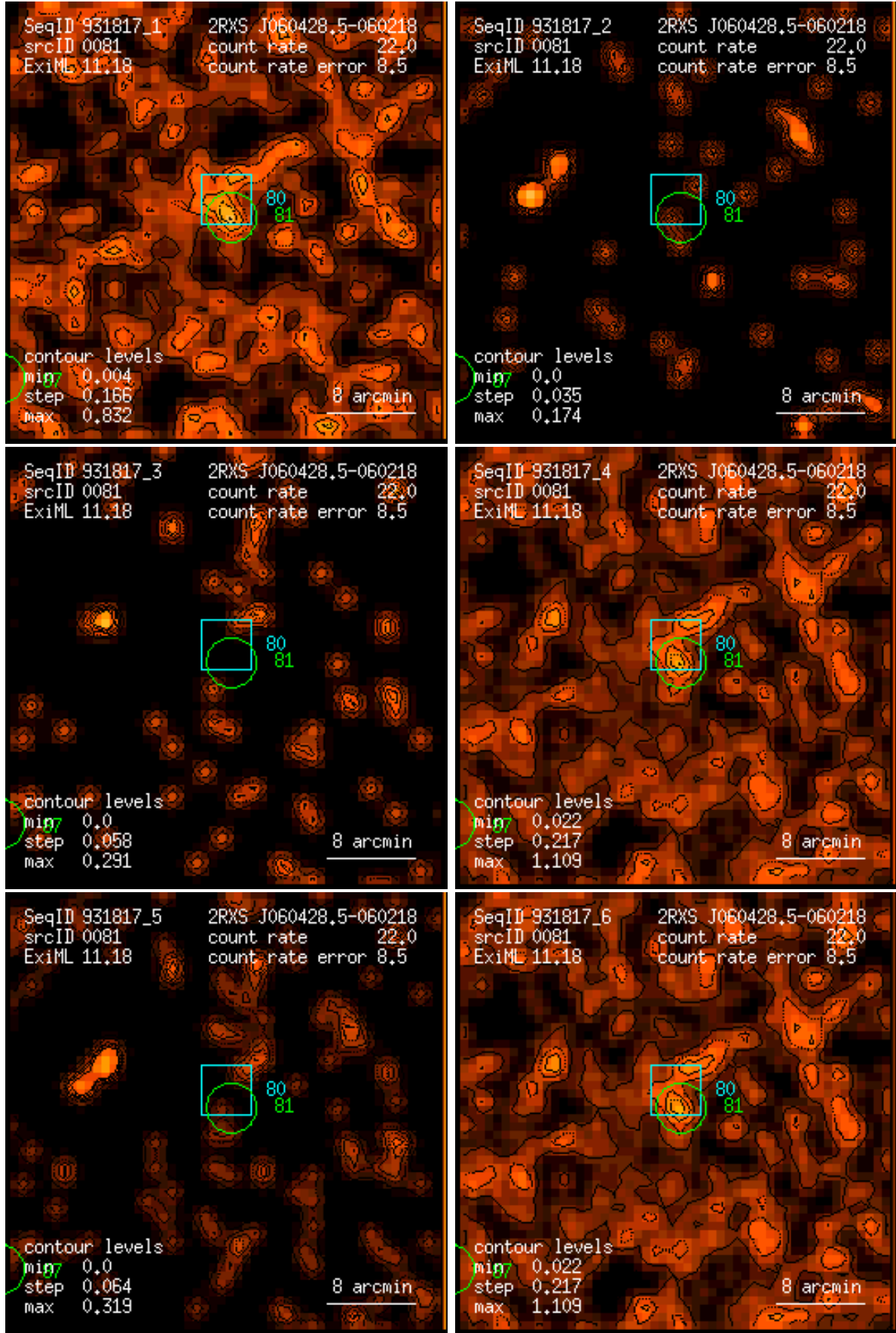
Figure 81: RASS 931817: detection 0081: band rate images, Gaussian filter: (1) PSPC channels 11 – 41, (2) 52 – 90, (3) 91 – 201, (4) 11 – 235, (5) 52 – 201, (6) 11 – 201. Broad band rates in counts/ks. Band rate contour levels in counts/ks/arcmin 2 .
