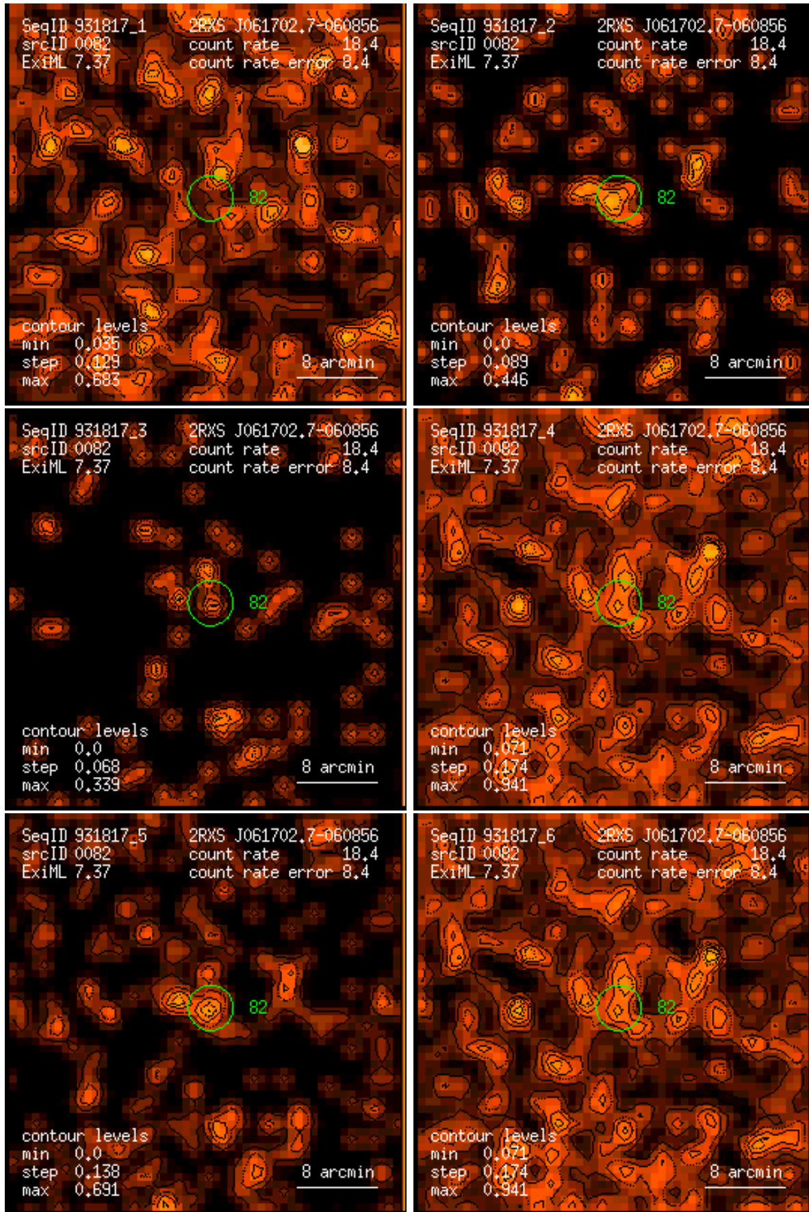
Figure 82: RASS 931817: detection 0082: band rate images, Gaussian filter: (1) PSPC channels 11 – 41, (2) 52 – 90, (3) 91 – 201, (4) 11 – 235, (5) 52 – 201, (6) 11 – 201. Broad band rates in counts/ks. Band rate contour levels in counts/ks/arcmin 2 .
